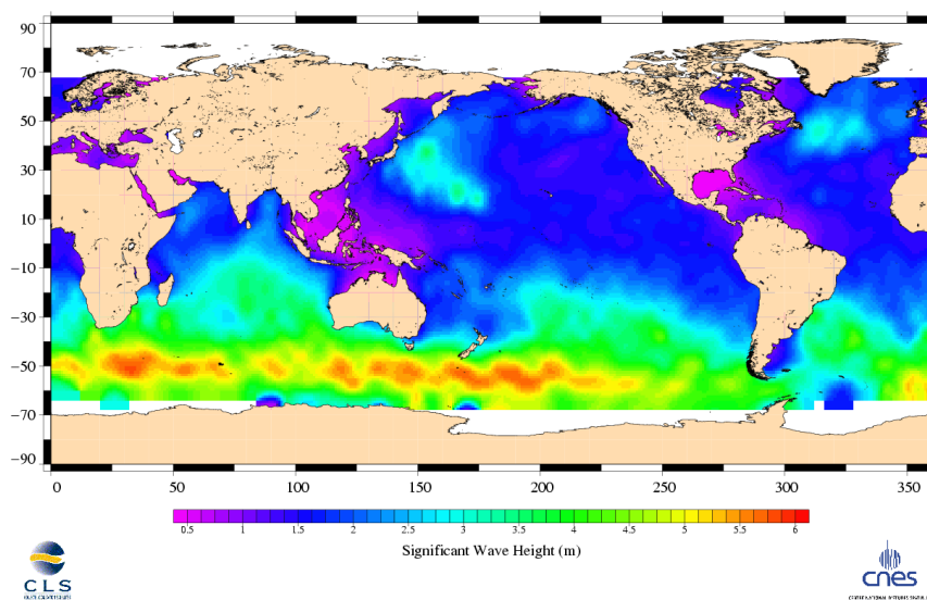
Jason-1 Cycle 171 27/08/2006 - 06/09/2006
