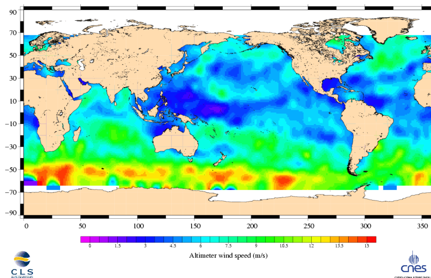
Jason-1 Cycle 171 27/08/2006 - 06/09/2006
