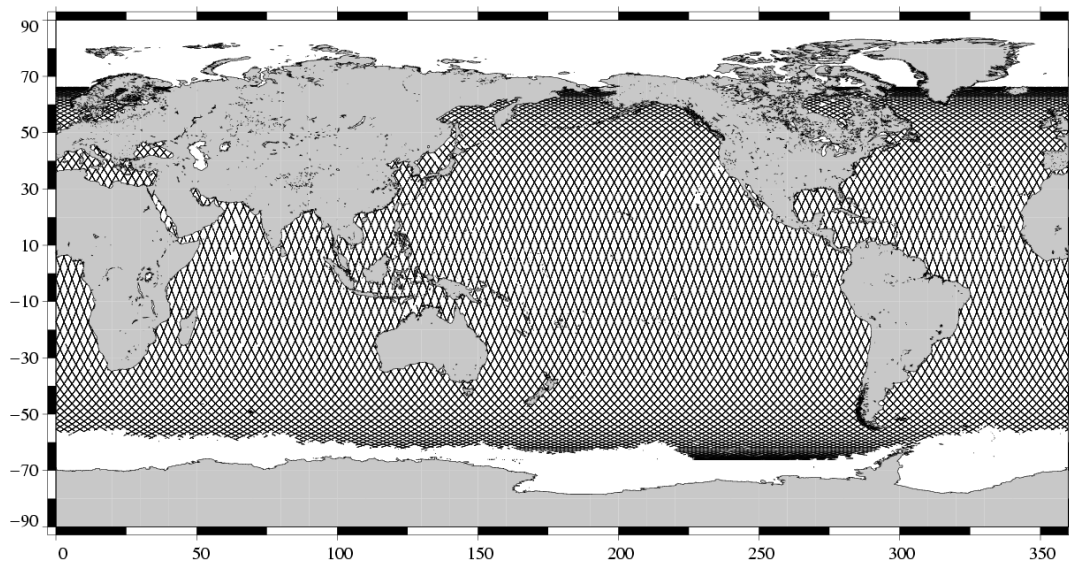
Valid data Jason-1 Cycle 174 (26/09/2006 / 06/10/2006)
