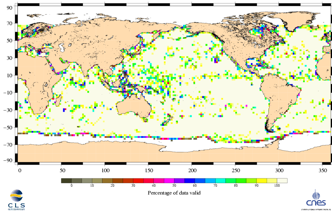
Percentage of valid data relative to the nominal pass Jason-1 Cycle 174 (26/09/2006 / 06/10/2006)
