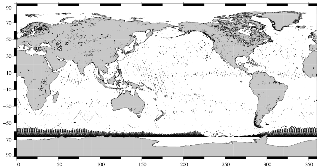
Edited measurements Jason-1 Cycle 174 (26/09/2006 / 06/10/2006)
