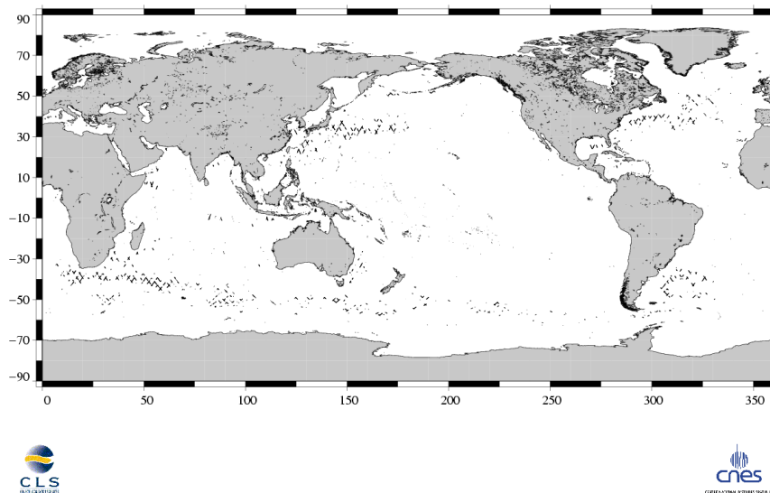
(SSH – MSS) differences greater than 30 cm Jason / Cycle 174
