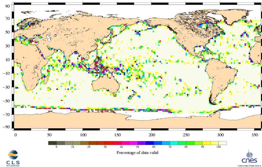
Percentage of valid data relative to the nominal pass Jason-1 Cycle 180 (25/11/2006 / 05/12/2006)
