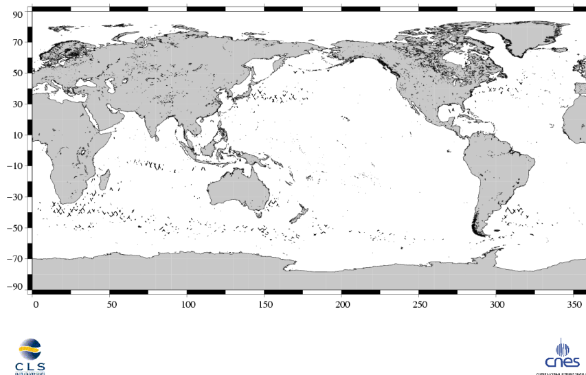
(SSH – MSS) differences greater than 30 cm Jason / Cycle 180
