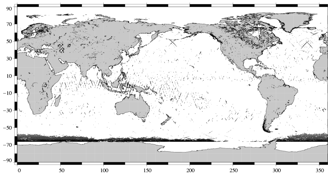
Edited measurements Jason-1 Cycle 180 (25/11/2006 / 05/12/2006)
