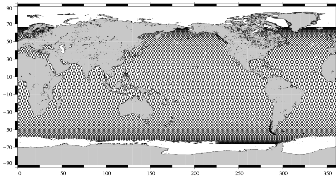
Valid data Jason-1 Cycle 180 (25/11/2006 / 05/12/2006)
