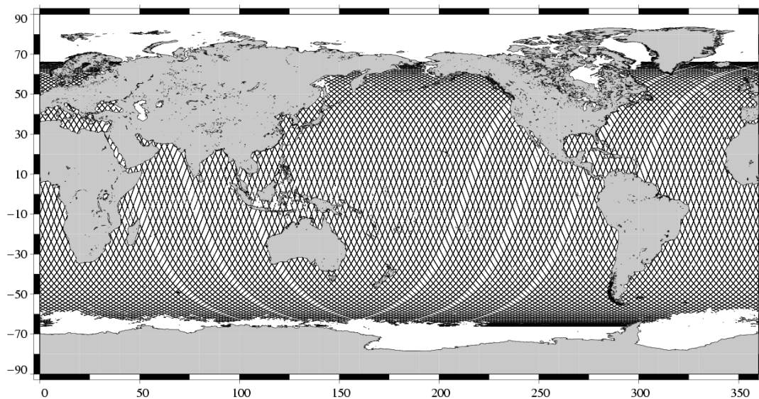
Valid data Jason-1 Cycle 181 (05/12/2006 / 14/12/2006)
