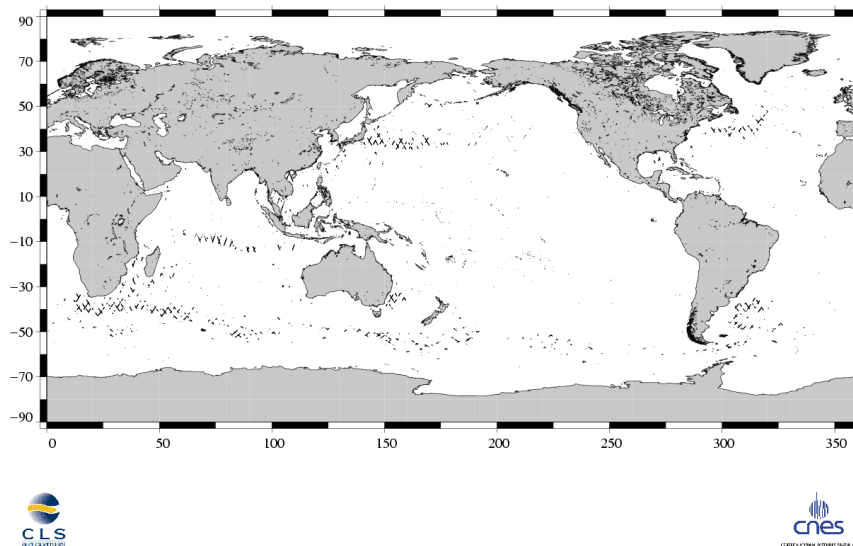
(SSH – MSS) differences greater than 30 cm Jason / Cycle 181
