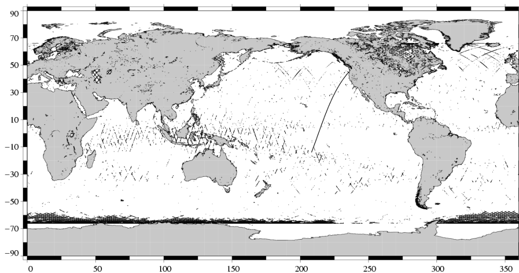
Edited measurements Jason-1 Cycle 181 (05/12/2006 / 14/12/2006)
