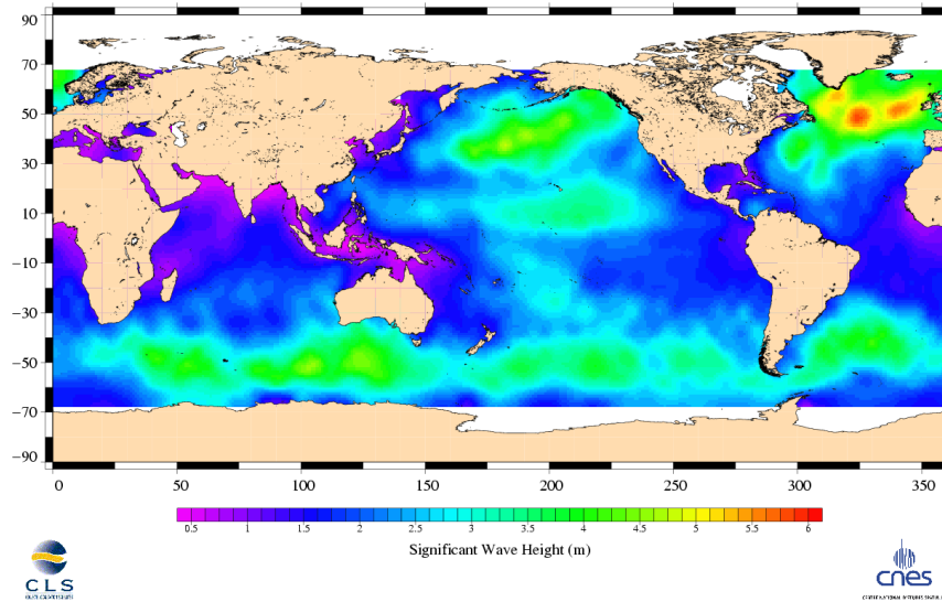
Jason-1 Cycle 185 13/01/2007 – 23/01/2007
