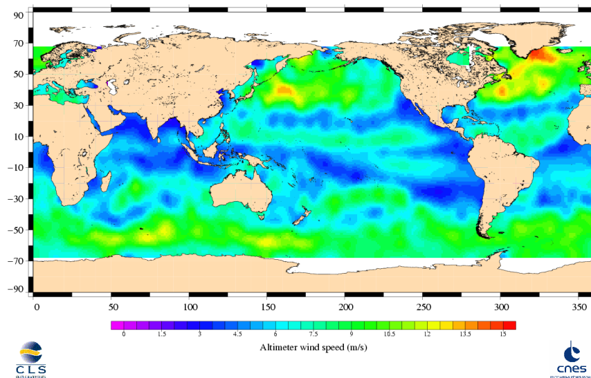
Jason-1 Cycle 187 02/02/2007 - 12/02/2007
