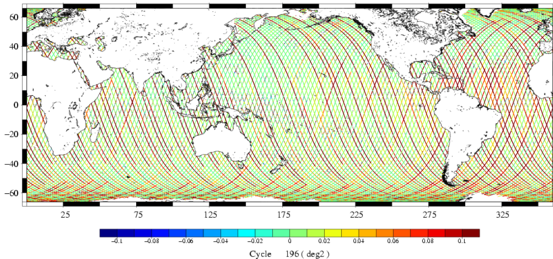
ATT_FO_CARRE [deg 2 ] J1 cycle 196
