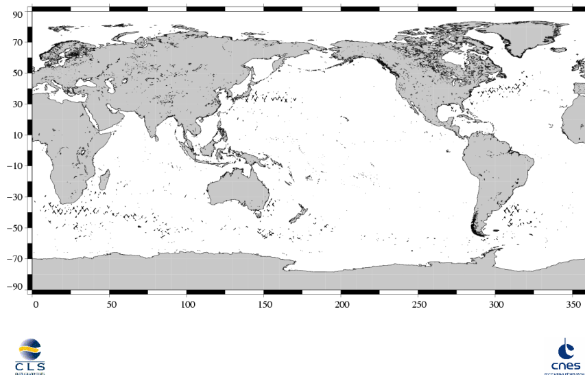
(SSH – MSS) differences greater than 30 cm Jason / Cycle 196
