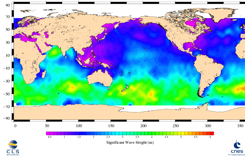
Jason-1 Cycle 201 21/06/2007 - 01/07/2007
