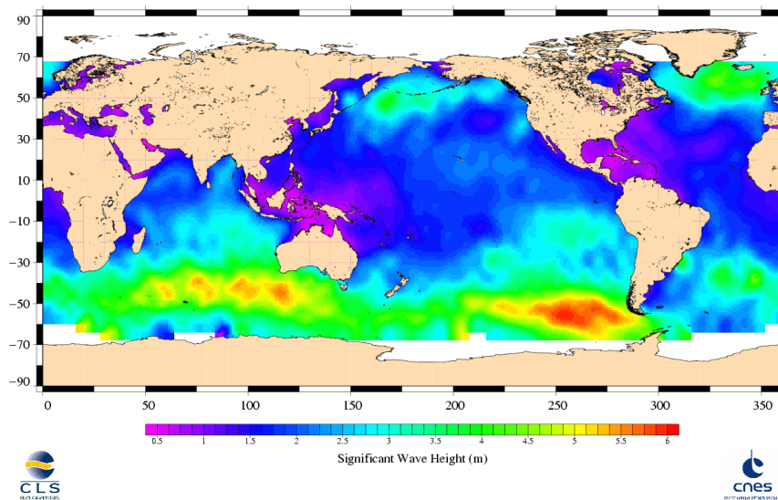
Jason-1 Cycle 210 18/09/2007 - 28/09/2007
