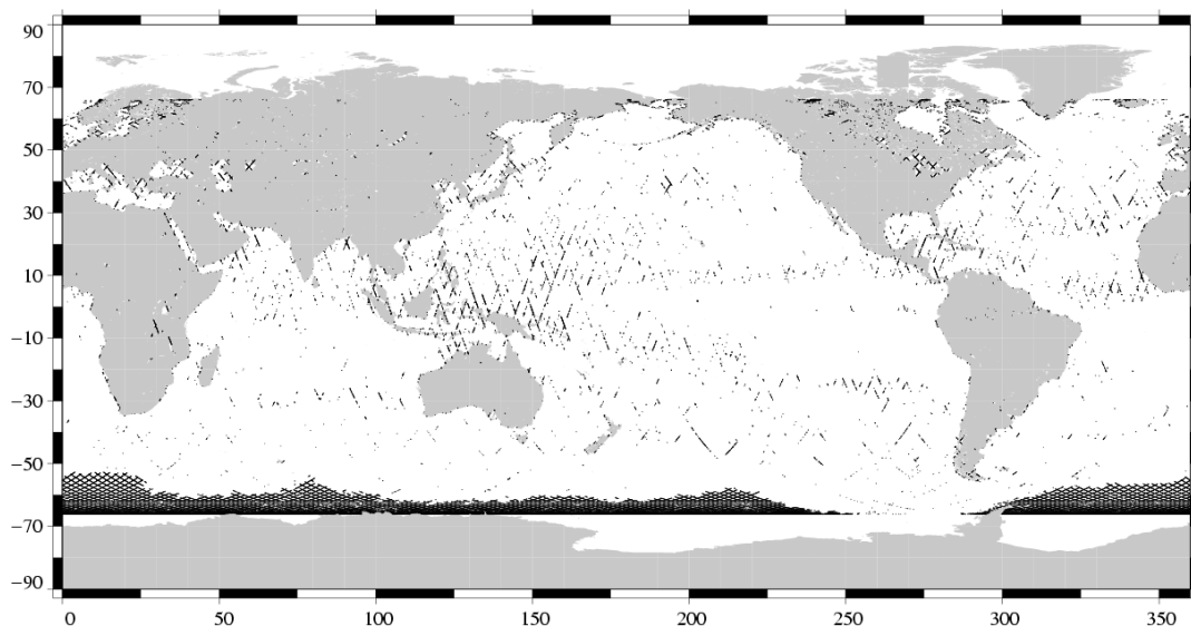
Edited measurements Jason-1 Cycle 211 (28/09/2007 / 08/10/2007)
