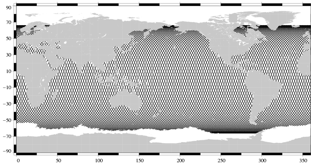
Valid data Jason-1 Cycle 211 (28/09/2007 / 08/10/2007)
