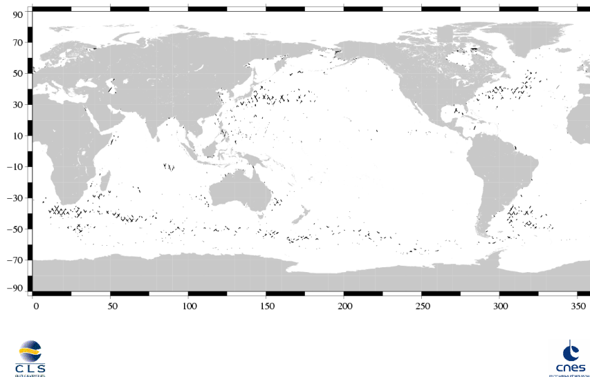
(SSH – MSS) differences greater than 30 cm Jason / Cycle 211
