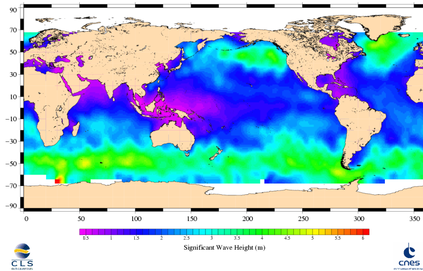
Jason-1 Cycle 212 08/10/2007 - 18/10/2007
