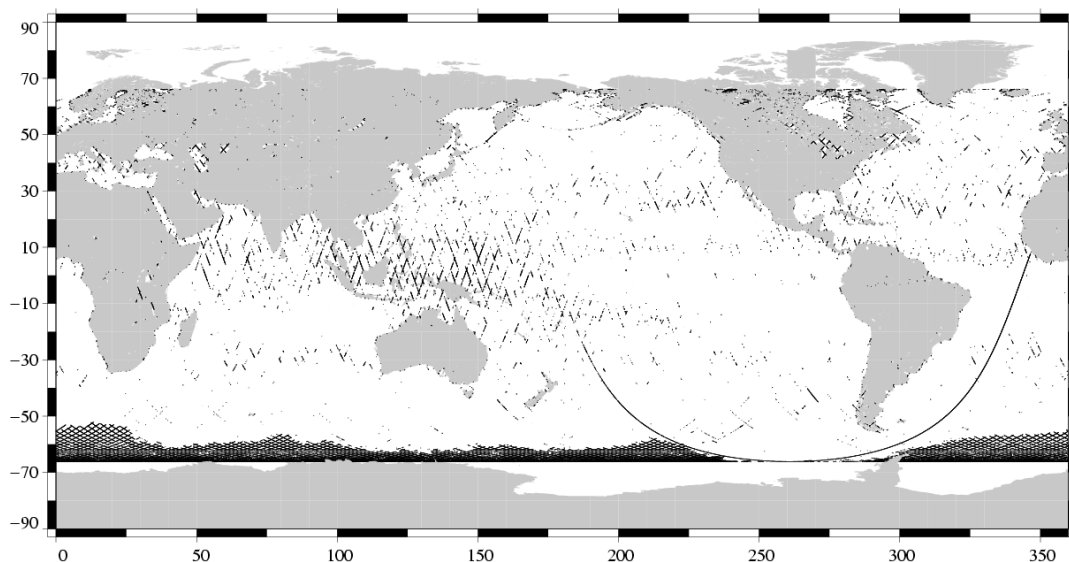
Edited measurements Jason-1 Cycle 212 (08/10/2007 / 18/10/2007)
