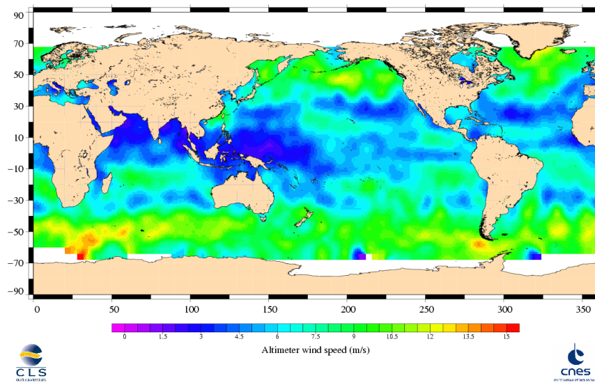
Jason-1 Cycle 212 08/10/2007 - 18/10/2007
