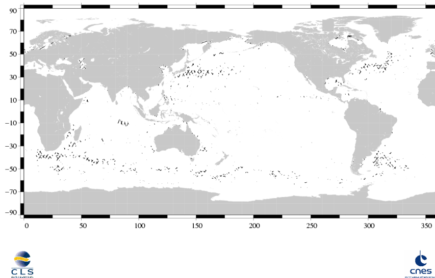
(SSH - MSS) differences greater than 30 cm Jason / Cycle 212
