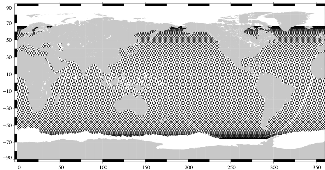
Valid data Jason-1 Cycle 212 (08/10/2007 / 18/10/2007)
