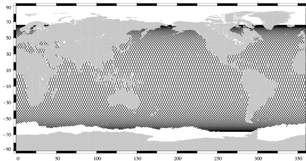
Valid data Jason-1 Cycle 213 (18/10/2007 / 28/10/2007)
