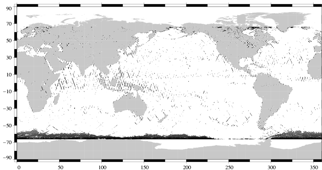
Edited measurements Jason-1 Cycle 215 (07/11/2007 / 17/11/2007)
