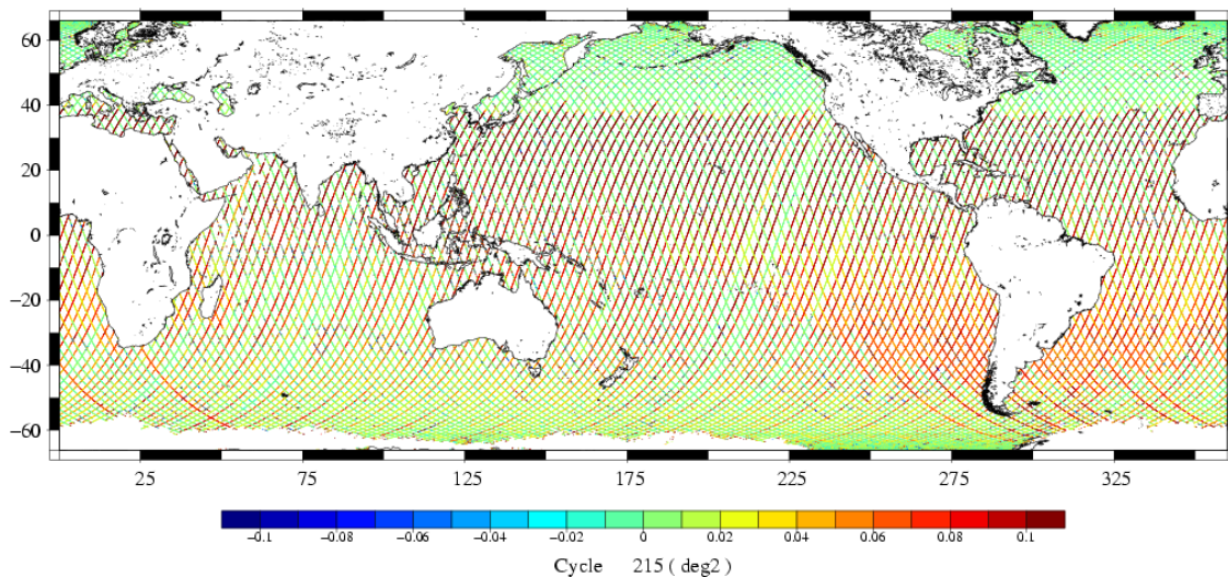
ATT_FO_CARRE [deg 2 ] J1 cycle 215
