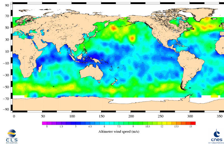
Jason-1 Cycle 217 26/11/2007 - 06/12/2007
