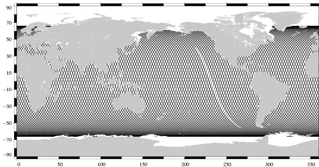
Valid data Jason-1 Cycle 222 (15/01/2008 / 25/01/2008)
