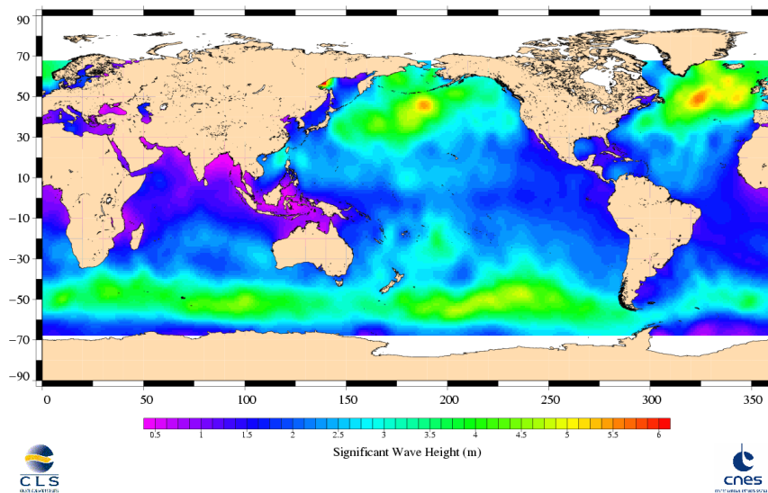
Jason-1 Cycle 222 15/01/2008 – 25/01/2008
