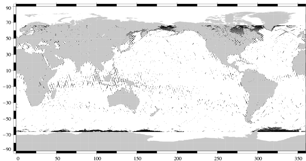
Edited measurements Jason-1 Cycle 222 (15/01/2008 / 25/01/2008)
