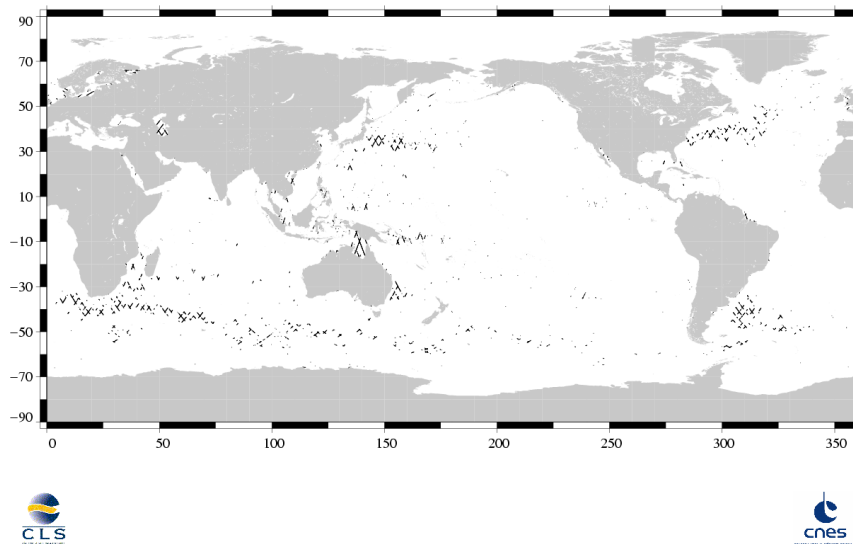
(SSH – MSS) differences greater than 30 cm Jason / Cycle 222
