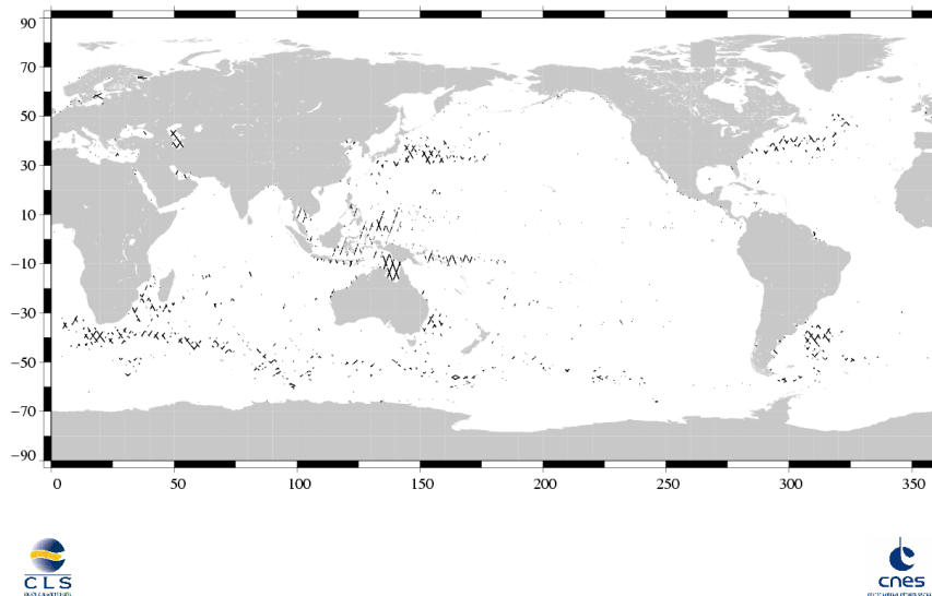
(SSH – MSS) differences greater than 30 cm Jason / Cycle 225
