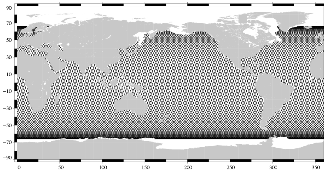
Valid data Jason-1 Cycle 226 (24/02/2008 / 05/03/2008)
