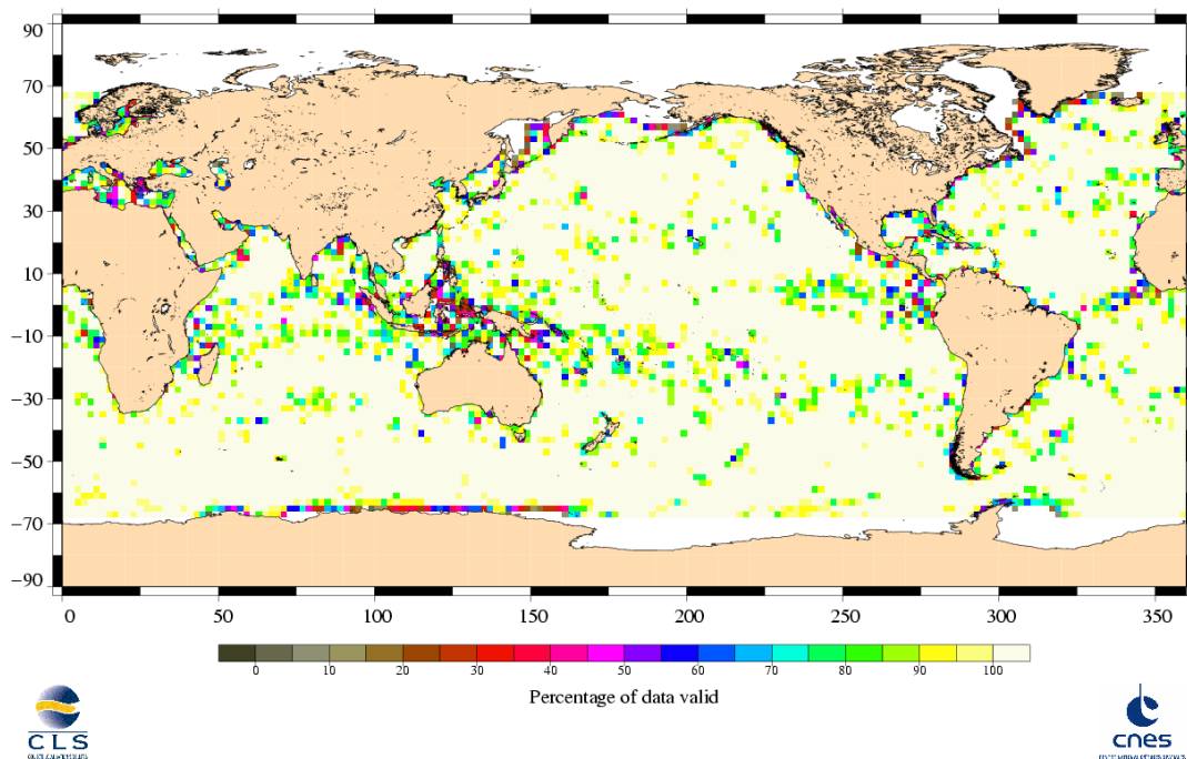
Percentage of valid data relative to the nominal pass Jason-1 Cycle 226 (24/02/2008 / 05/03/2008)
