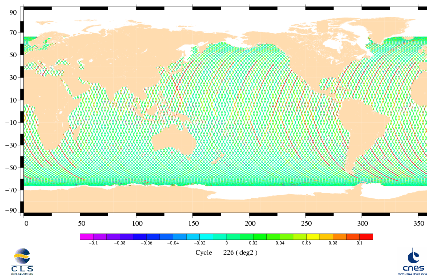
Square of the off nadir angle from waveforms Jason-1 Cycle 226 (24/02/2008 / 05/03/2008)
