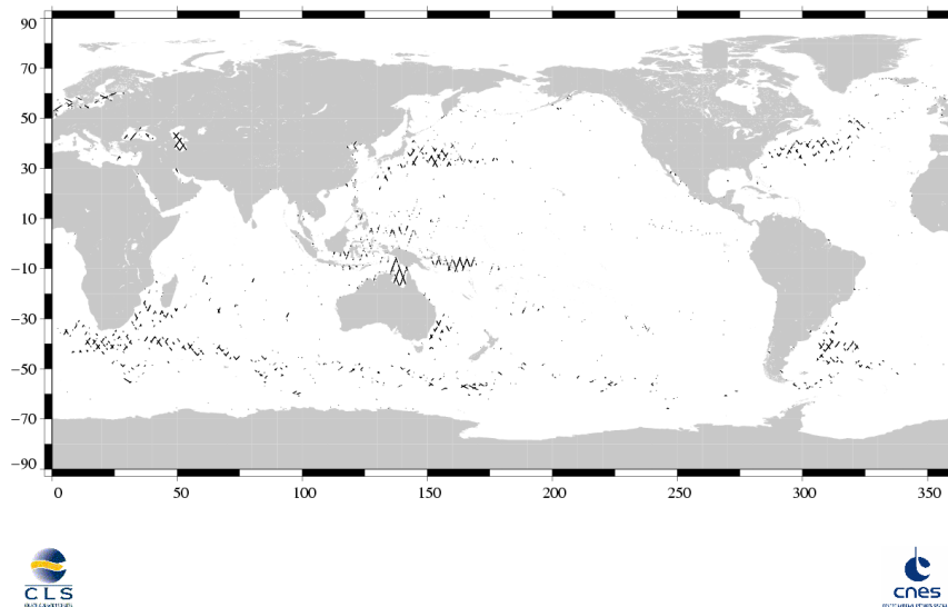
(SSH – MSS) differences greater than 30 cm Jason / Cycle 226
