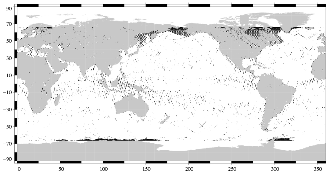
Edited measurements Jason-1 Cycle 226 (24/02/2008 / 05/03/2008)
