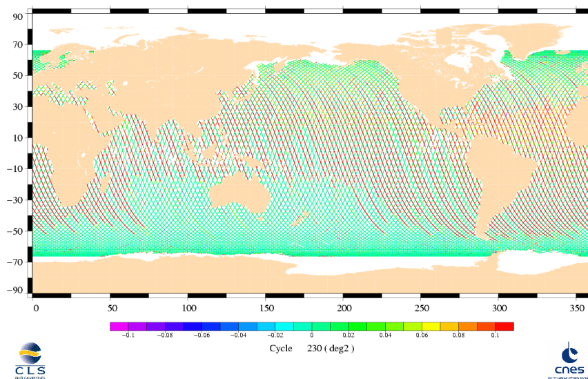
Square of the off nadir angle from waveforms Jason-1 Cycle 230 (03/04/2008 / 13/04/2008)
