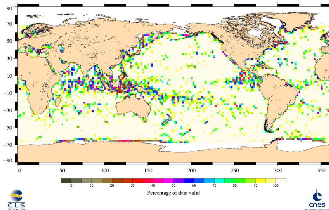
Percentage of valid data relative to the nominal pass Jason-1 Cycle 230 (03/04/2008 / 13/04/2008)
