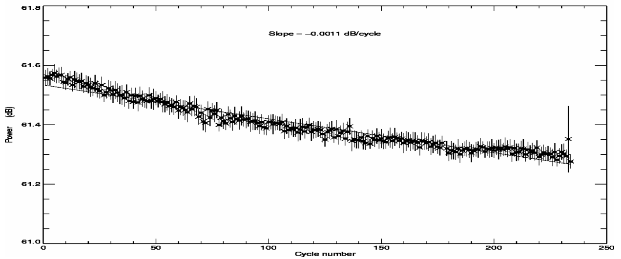
POSEIDON2 – Cycle 234
