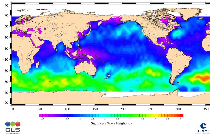
Jason-1 Cycle 234 13/05/2008 – 23/05/2008
