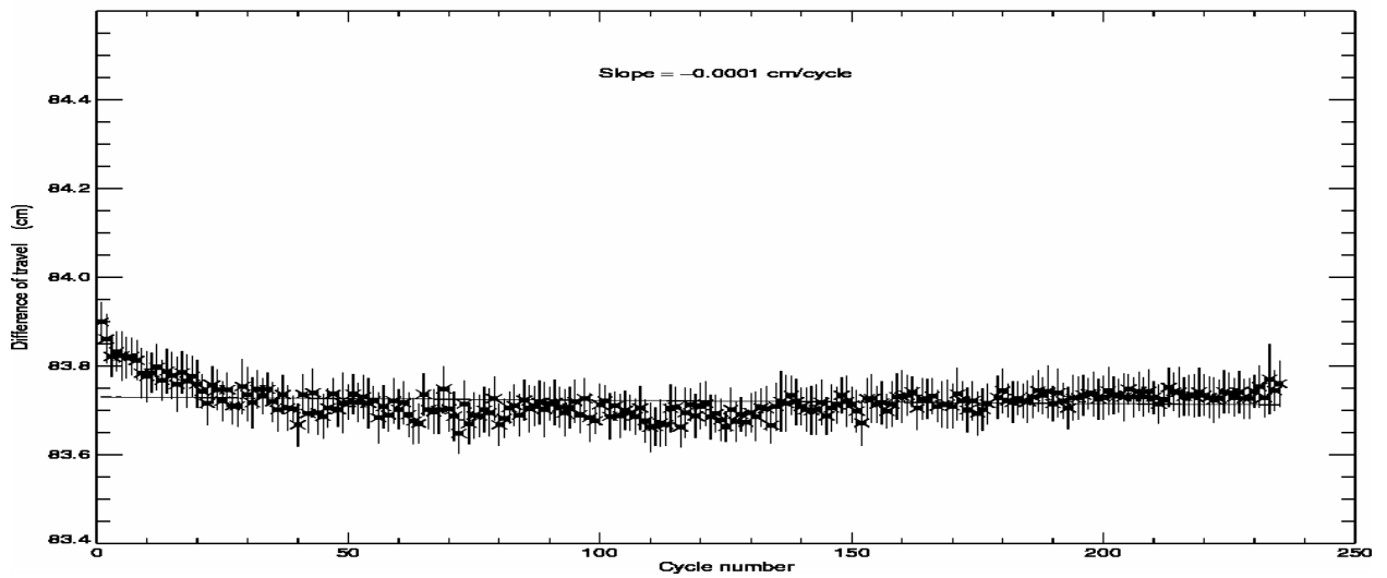
POSEIDON2 – Cycle 235 Difference of travel between E and R lines of the PTR in C band
