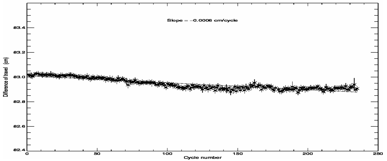
POSEIDON2 – Cycle 235 Difference of travel between E and R lines of the PTR in C band
