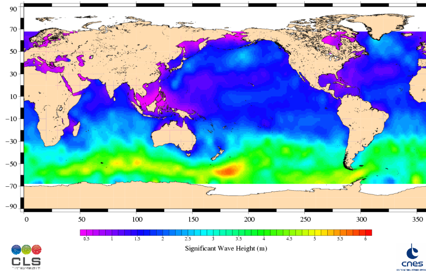
Jason-1 Cycle 235 23/05/2008 – 02/06/2008
