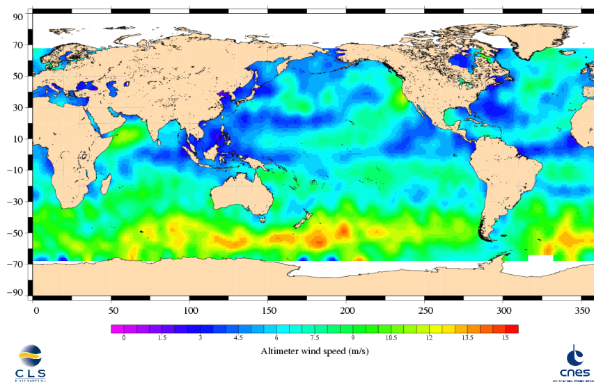
Jason-1 Cycle 236 02/06/2008 - 12/06/2008
