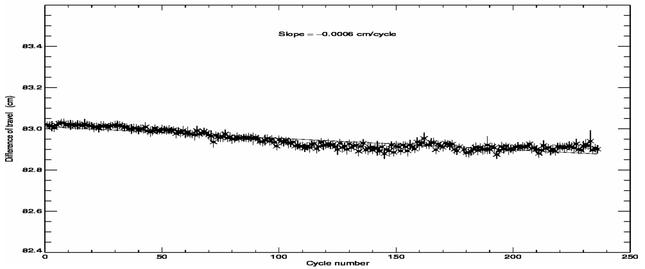
POSEIDON2 – Cycle 236 Difference of travel between E and R lines of the PTR in C band
