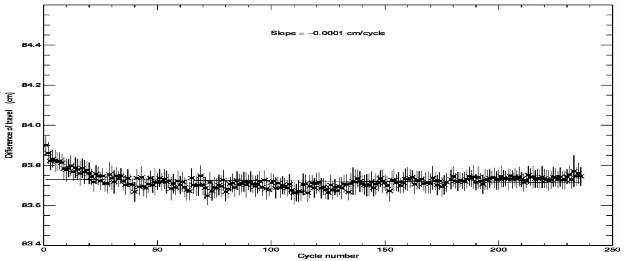
POSEIDON2 – Cycle 236 Difference of travel between E and R lines of the PTR in C band
