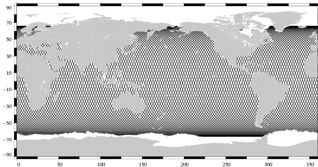
Valid data Jason-1 Cycle 236 (02/06/2008 / 12/06/2008)
