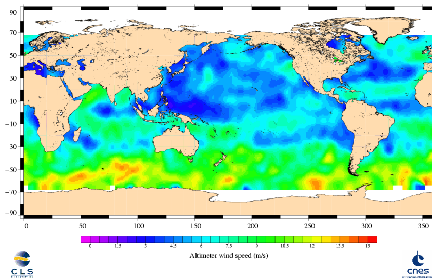
Jason-1 Cycle 239 02/07/2008 - 12/07/2008
