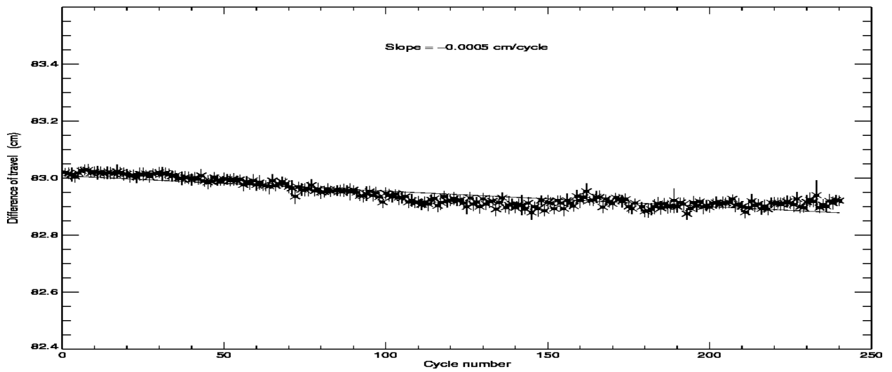
POSEIDON2 – Cycle 240 Difference of travel between E and R lines of the PTR in C band
