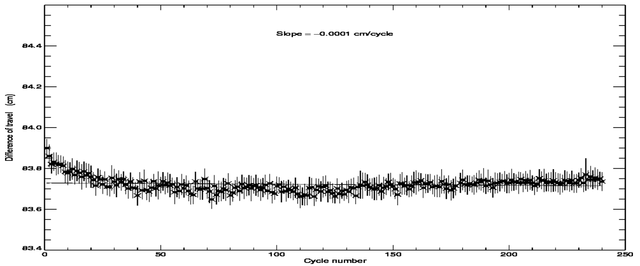
POSEIDON2 – Cycle 240 Difference of travel between E and R lines of the PTR in C band
