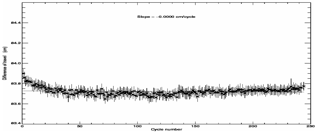
POSEIDON2 – Cycle 244 Difference of travel between E and R lines of the PTR in C band
