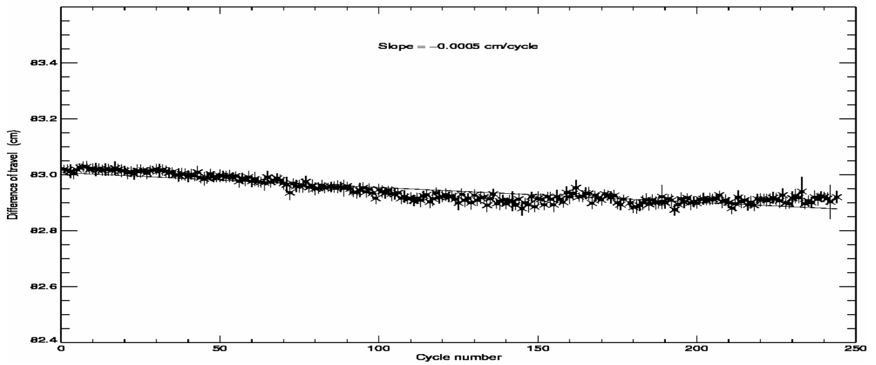
POSEIDON2 – Cycle 244 Difference of travel between E and R lines of the PTR in C band
