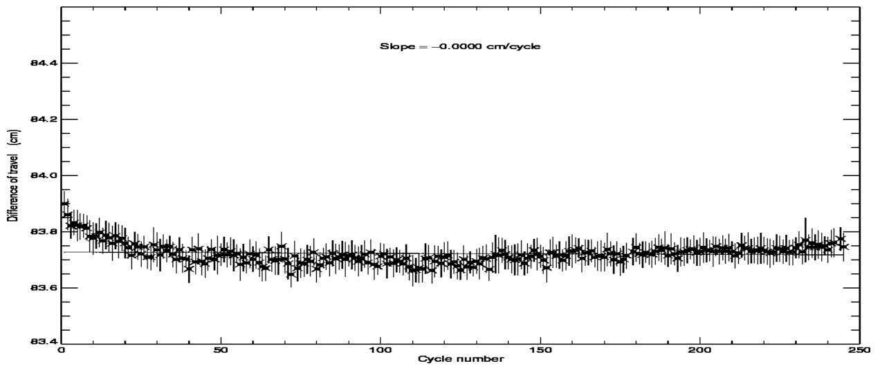
POSEIDON2 – Cycle 245 Difference of travel between E and R lines of the PTR in C band
