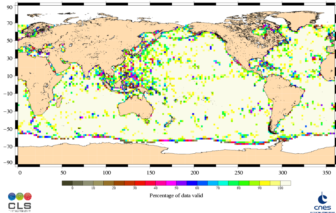
Percentage of valid data relative to the nominal pass Jason-1 Cycle 245 (30/08/2008 / 09/09/2008)
