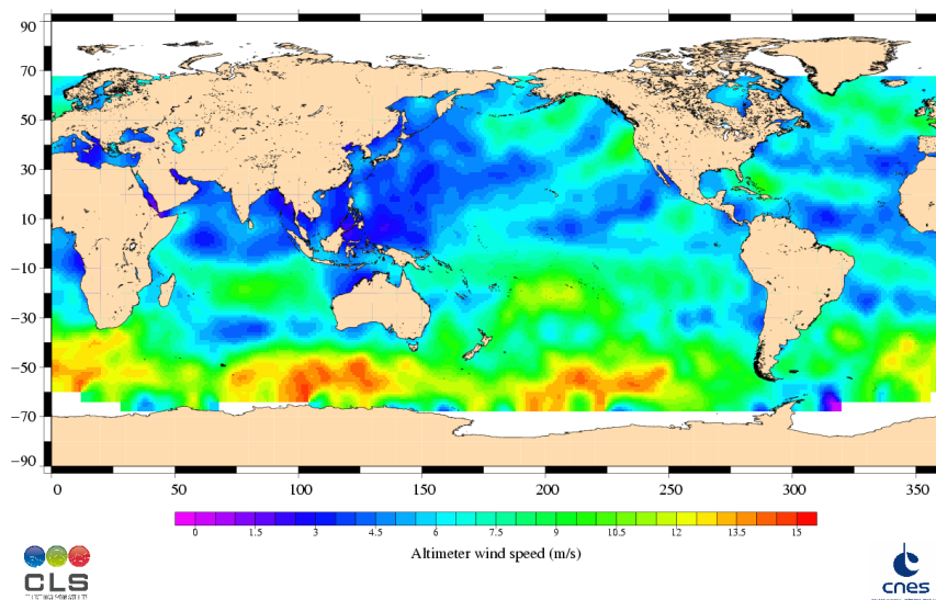
Jason-1 Cycle 245 30/08/2008 - 09/09/2008
