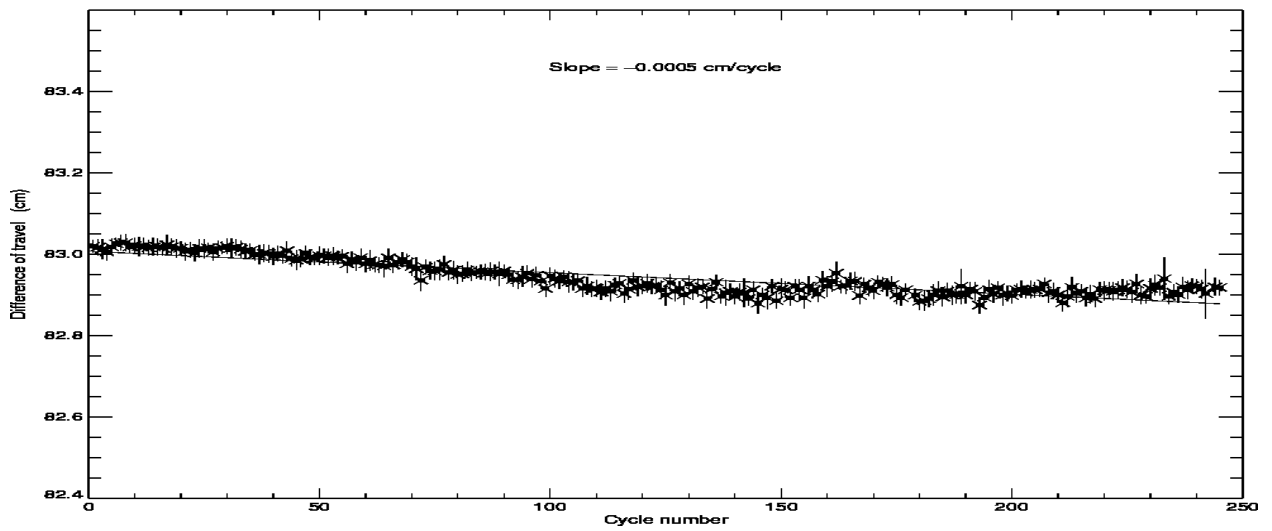
POSEIDON2 – Cycle 245 Difference of travel between E and R lines of the PTR in C band
