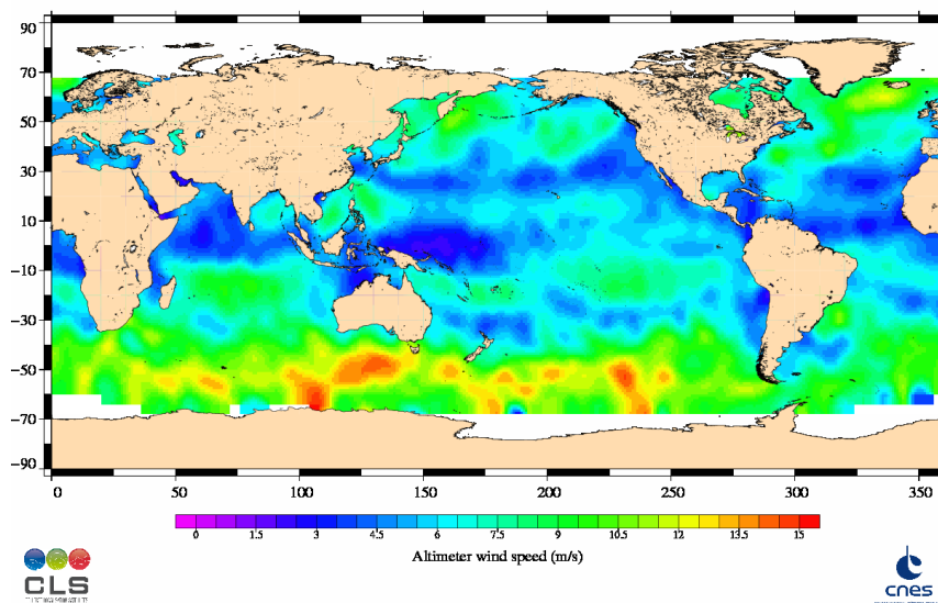
Jason-1 Cycle 247 19/09/2008 - 29/09/2008
