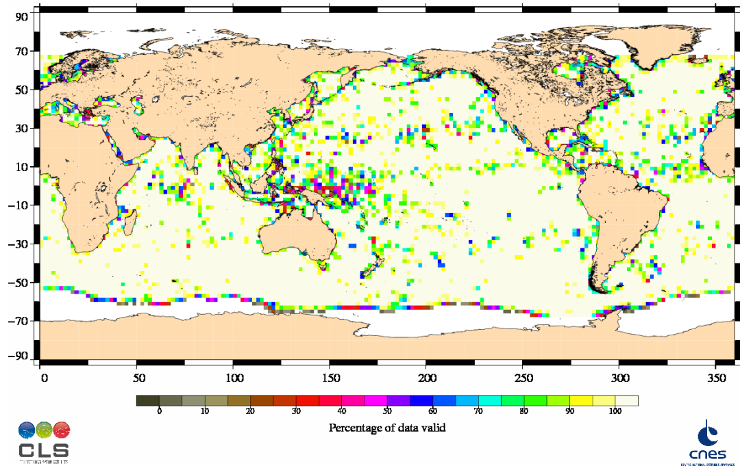
Percentage of valid data relative to the nominal pass Jason-1 Cycle 247 (19/09/2008 / 29/09/2008)
