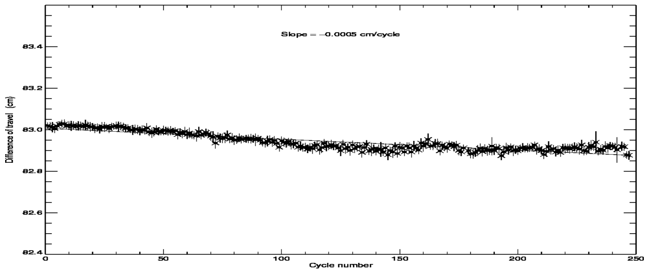
POSEIDON2 – Cycle 247 Difference of travel between E and R lines of the PTR in C band
