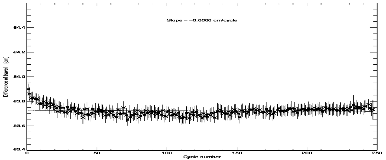
POSEIDON2 – Cycle 247 Difference of travel between E and R lines of the PTR in C band
