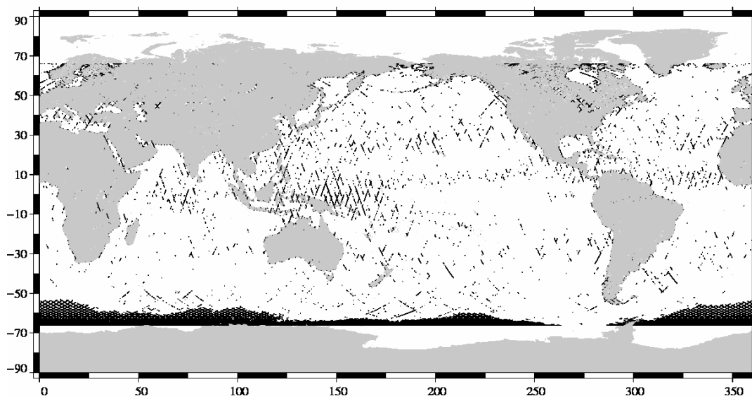
Edited measurements Jason-1 Cycle 247 (19/09/2008 / 29/09/2008)
