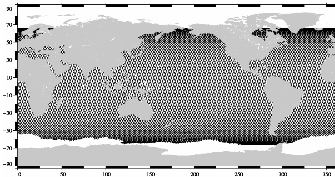
Valid data Jason-1 Cycle 247 (19/09/2008 / 29/09/2008)
