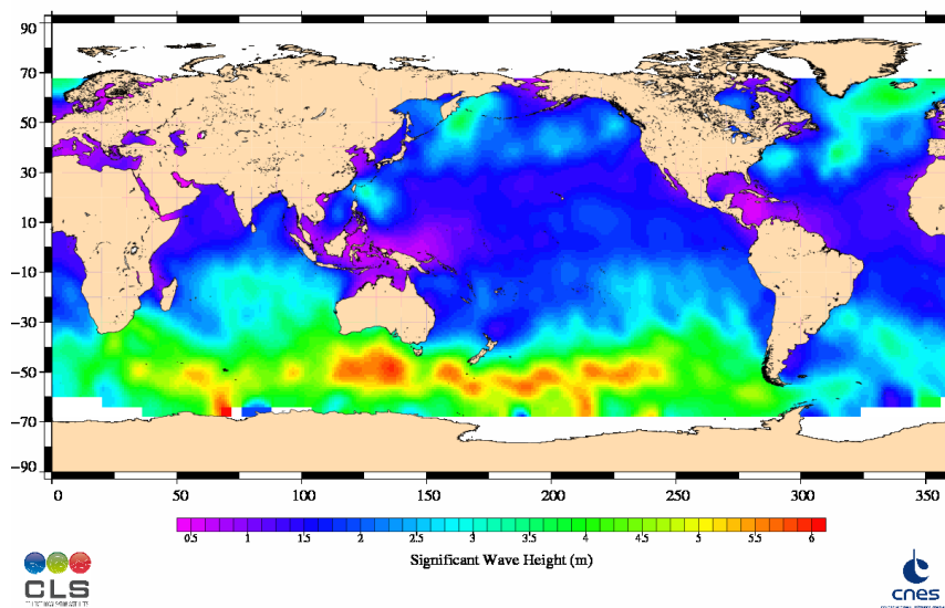
Jason-1 Cycle 247 19/09/2008 - 29/09/2008
