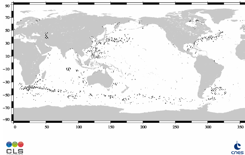
(SSH – MSS) differences greater than 30 cm Jason / Cycle 247
