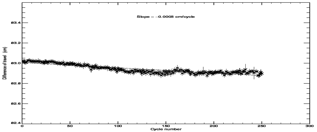
POSEIDON2 – Cycle 250 Difference of travel between E and R lines of the PTR in C band
