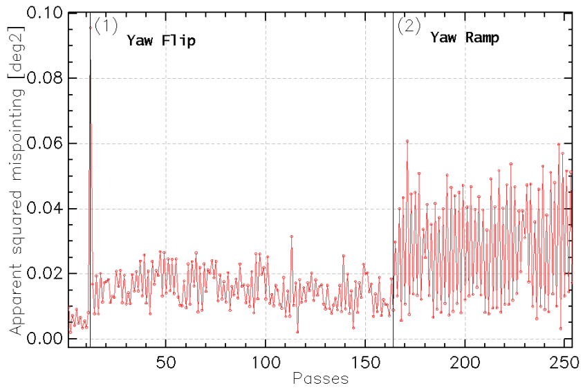
Mean per pass of apparent squared mispointing of Jason-1 cycle 250
