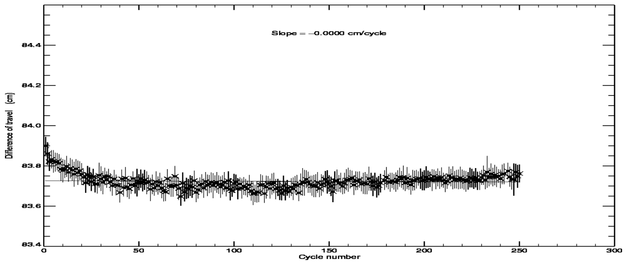
POSEIDON2 – Cycle 250 Difference of travel between E and R lines of the PTR in C band
