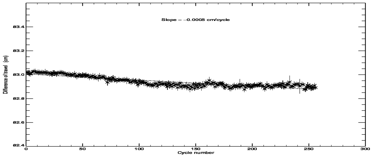
POSEIDON2 – Cycle 256 Difference of travel between E and R lines of the PTR in C band
