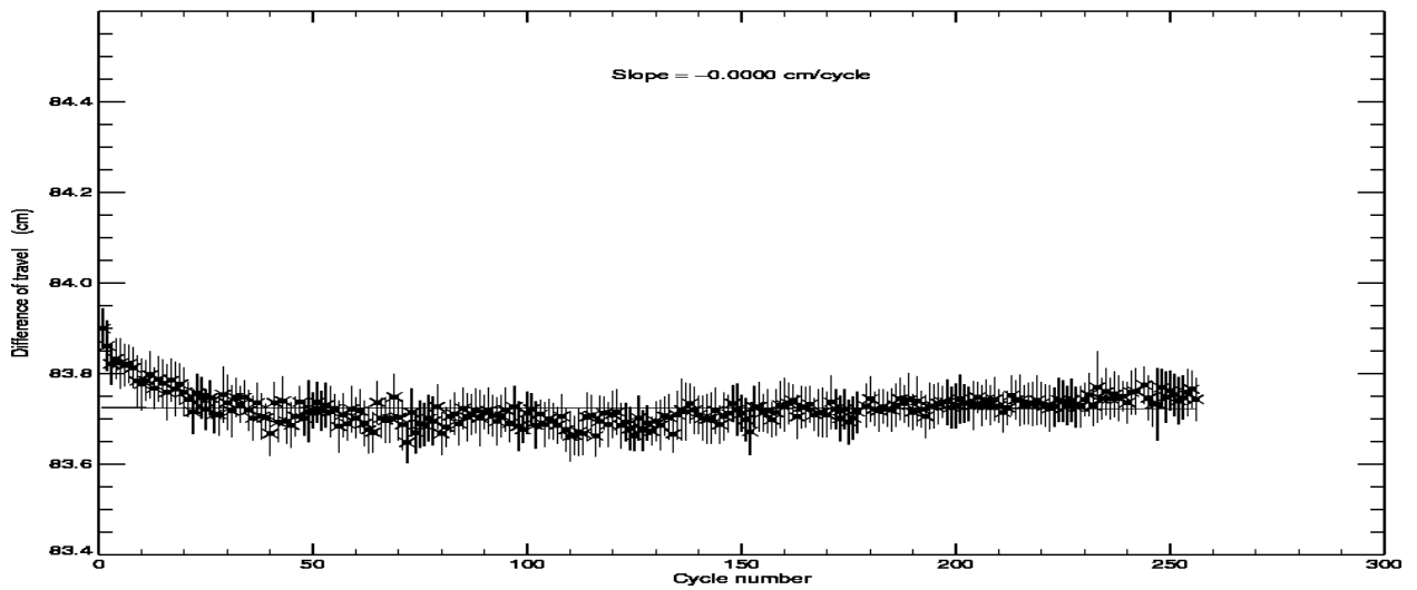
POSEIDON2 – Cycle 256 Difference of travel between E and R lines of the PTR in C band
