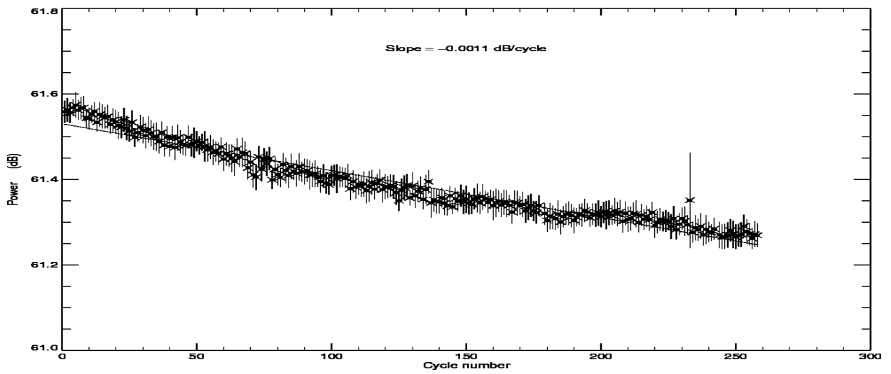
POSEIDON2 – Cycle 258 Total power of the PTR in C band
