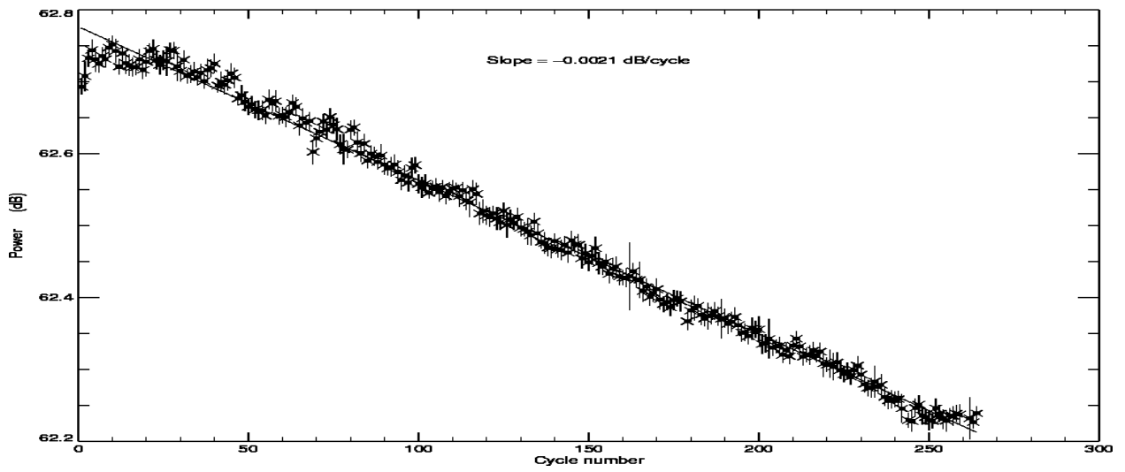
POSEIDON2 – Cycle 264 Total power of the PTR in C band
