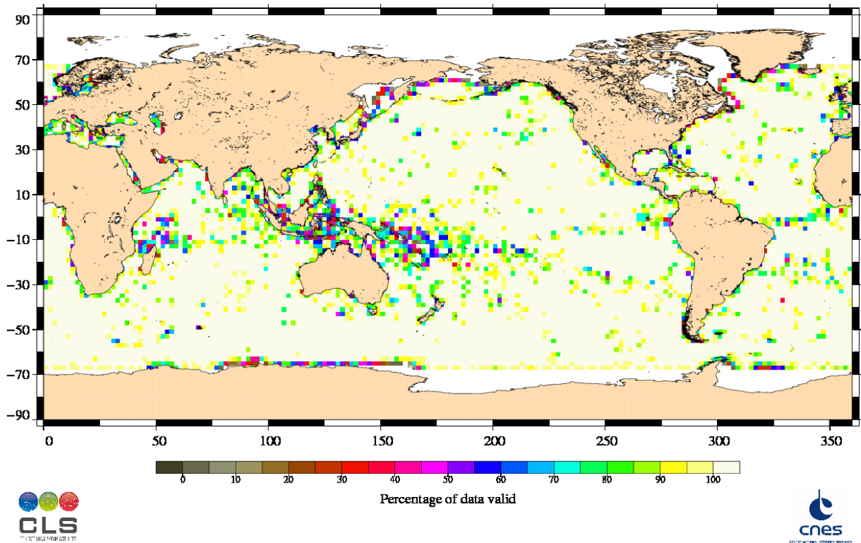
Percentage of valid data relative to the nominal pass Jason-1 Cycle 264 (02/03/2009 / 11/03/2009)
