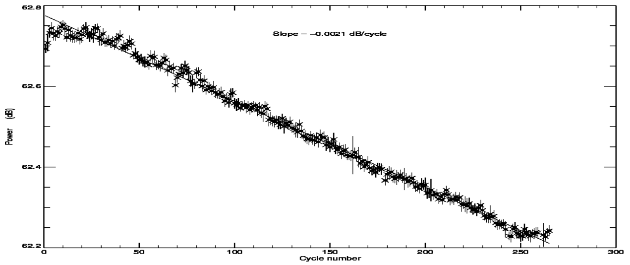
POSEIDON2 – Cycle 265 Total power of the PTR in C band
