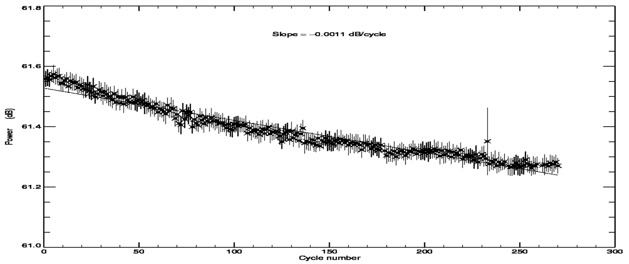
POSEIDON2 – Cycle 270 Total power of the PTR in C band
