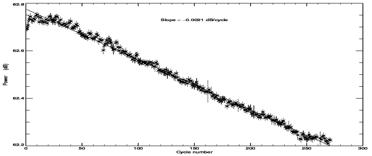
POSEIDON2 – Cycle 271 Total power of the PTR in C band
