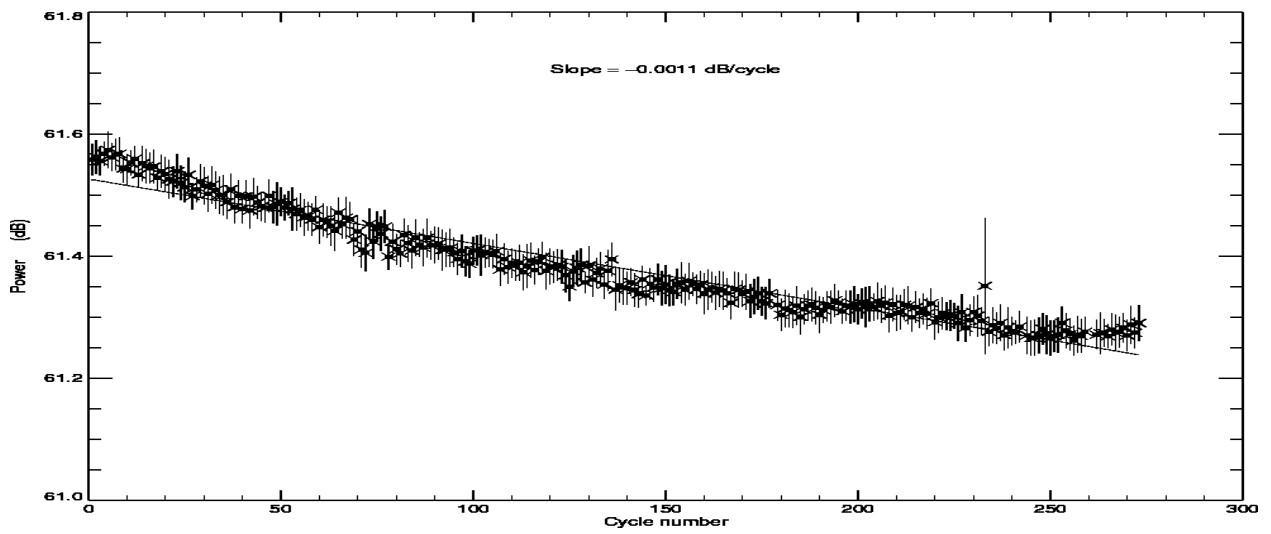
POSEIDON2 – Cycle 273 Total power of the PTR in C band
