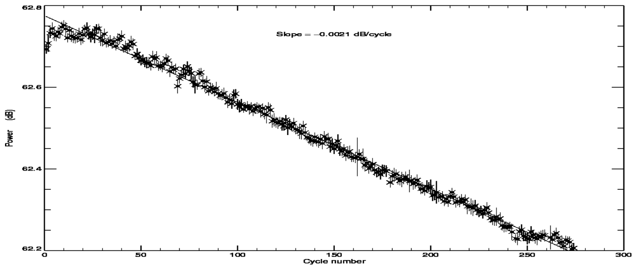
POSEIDON2 – Cycle 274 Total power of the PTR in C band
