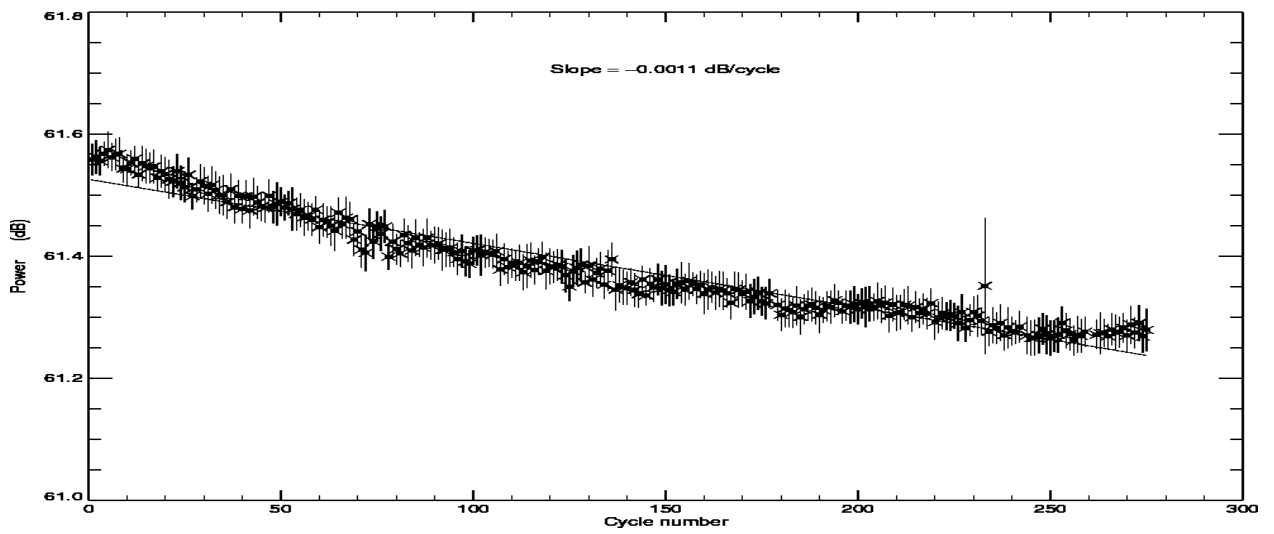
POSEIDON2 – Cycle 275 Total power of the PTR in C band
