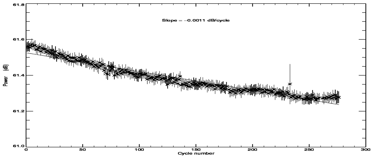
POSEIDON2 – Cycle 276 Total power of the PTR in C band
