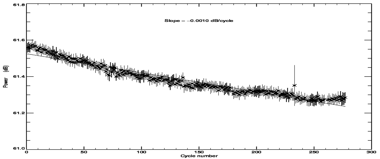
POSEIDON2 – Cycle 277 Total power of the PTR in C band
