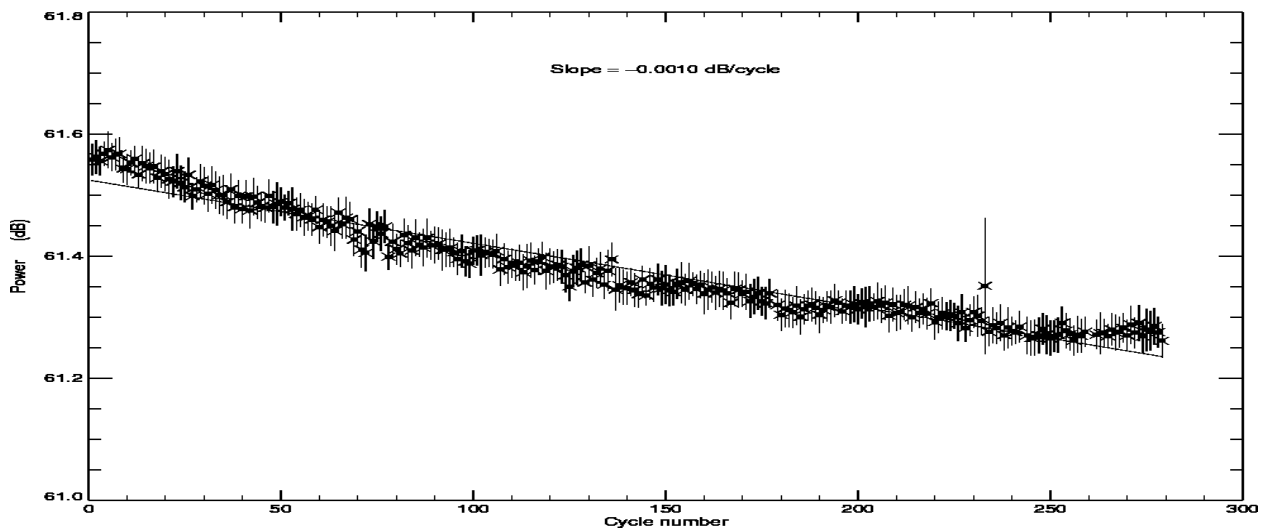
POSEIDON2 – Cycle 279 Total power of the PTR in C band
