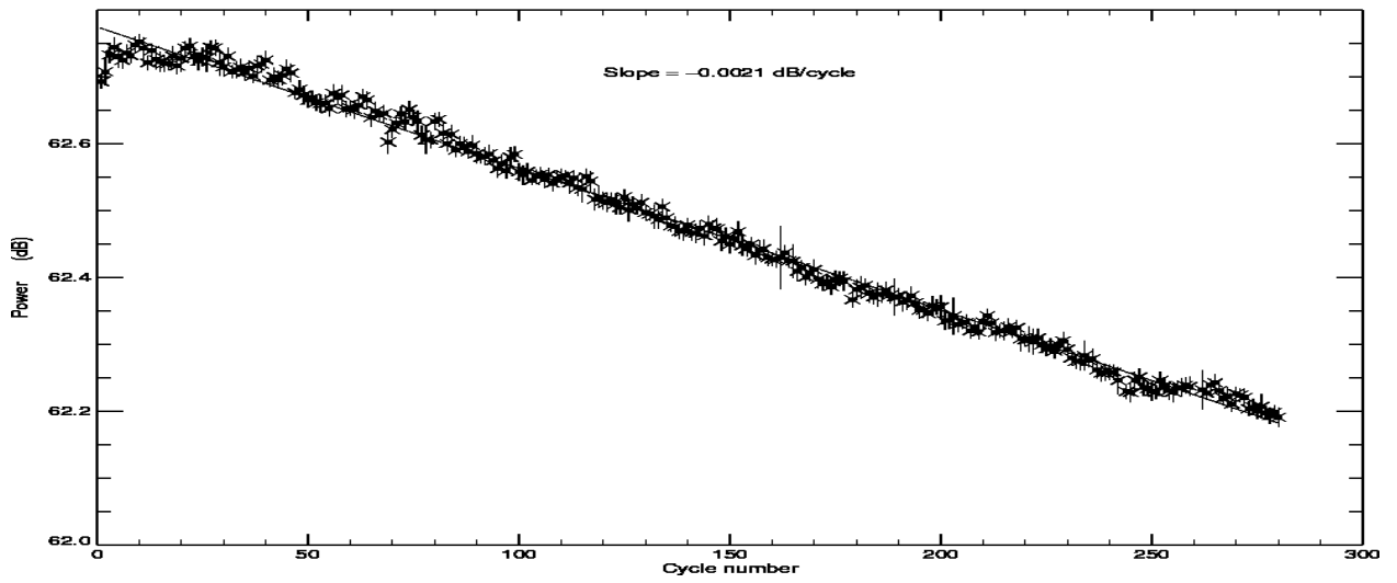
POSEIDON2 – Cycle 280 Total power of the PTR in C band
