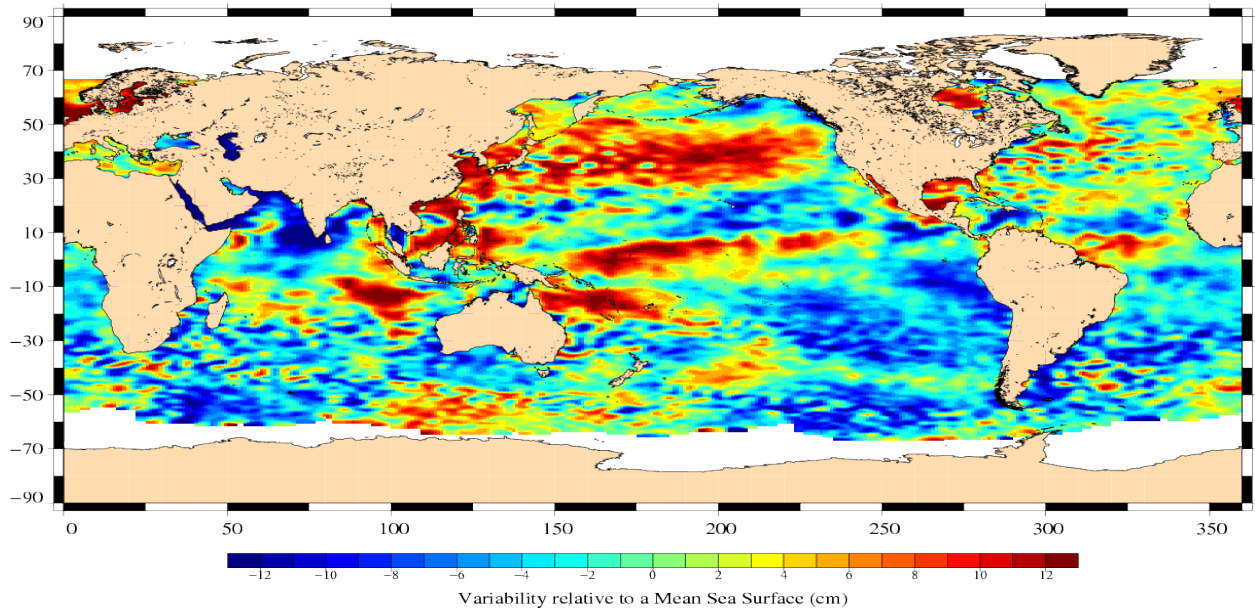
Jason-1 Cycle 285 26/09/2009 – 06/10/2009
