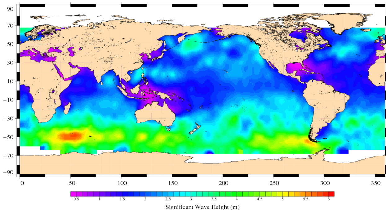
Jason-1 Cycle 285 26/09/2009 – 06/10/2009
