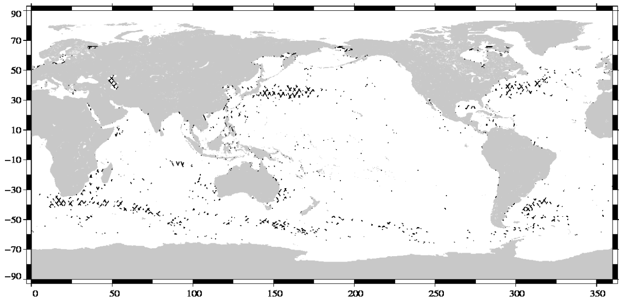
Valid data: (SSH – MSS) differences greater than 30 cm Jason-1 Cycle 287 (16/10/2009 / 26/10/2009)
