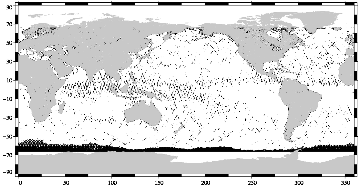
Valid data Jason-1 Cycle 287 (16/10/2009 / 26/10/2009)
