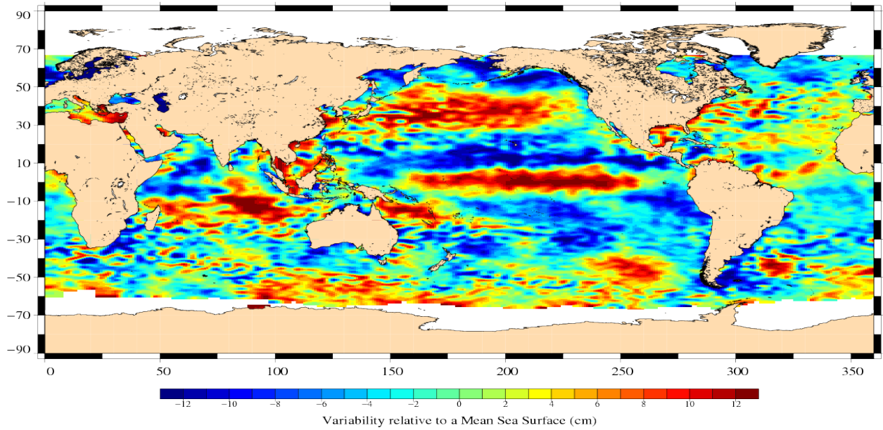
Jason-1 Cycle 289 04/11/2009 – 14/11/2009
