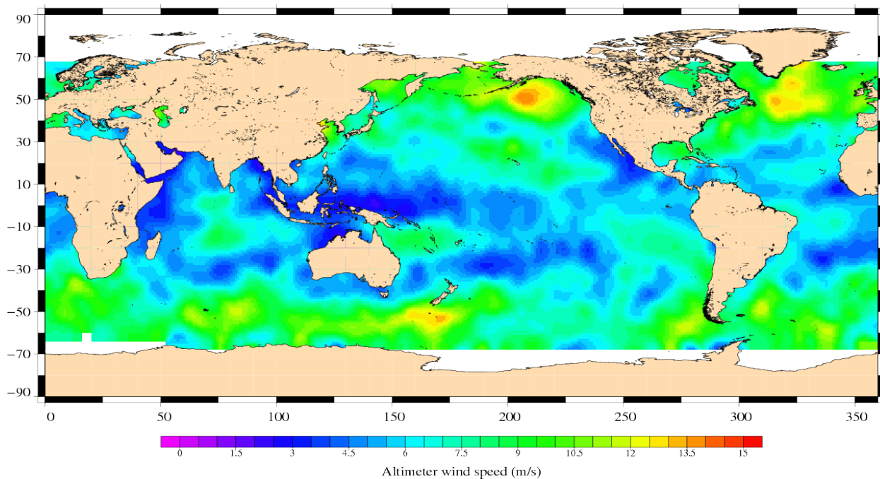
Jason-1 Cycle 289 04/11/2009 - 14/11/2009
