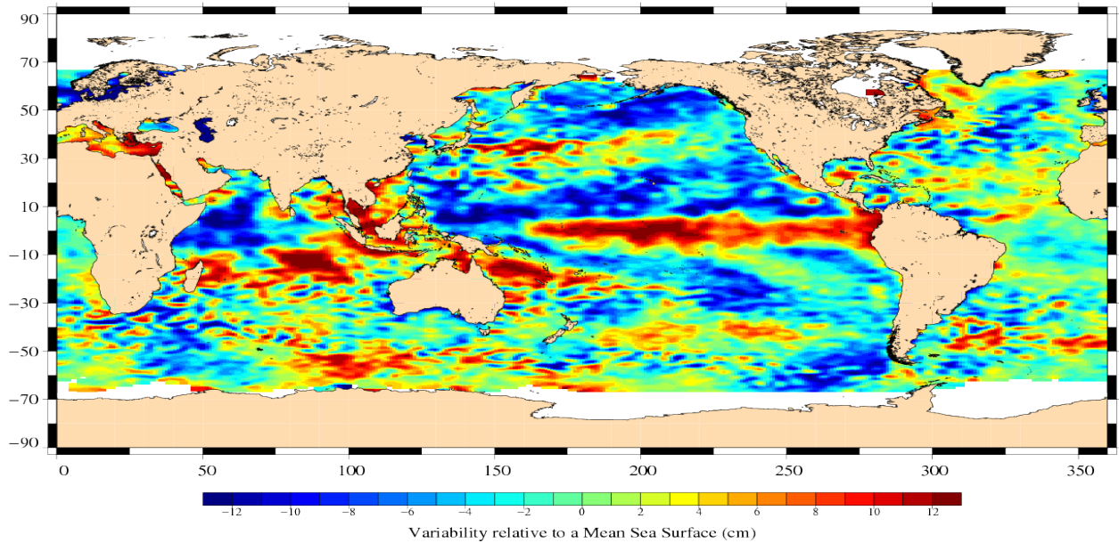
Jason-1 Cycle 293 14/12/2009 – 24/12/2009
