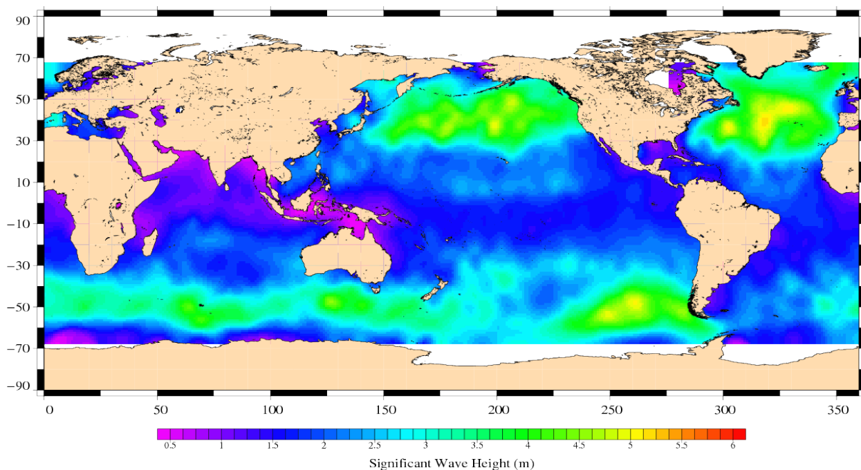
Jason-1 Cycle 293 14/12/2009 – 24/12/2009
