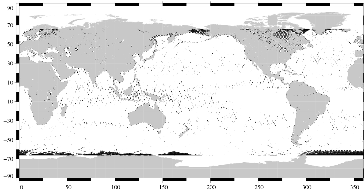
Valid data Jason-1 Cycle 294 (24/12/2009 / 03/01/2010)
