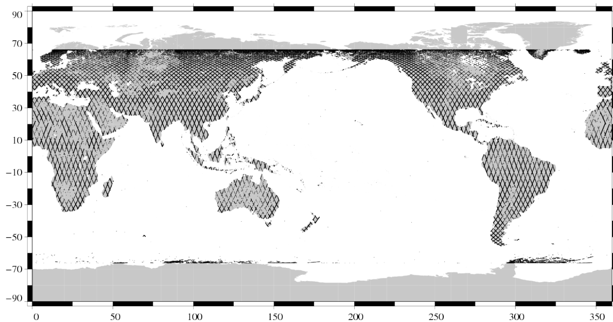
Missing measurements Jason-1 Cycle 294 (24/12/2009 / 03/01/2010)
