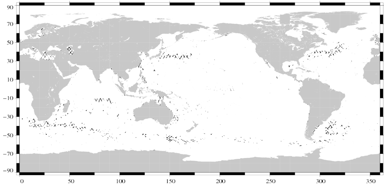
Valid data: (SSH – MSS) differences greater than 30 cm Jason-1 Cycle 294 (24/12/2009 / 03/01/2010)
