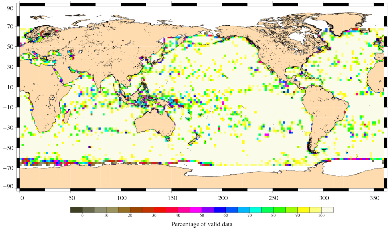
Percentage of valid data relative to the nominal pass Jason-1 Cycle 294 (24/12/2009 / 03/01/2010)
