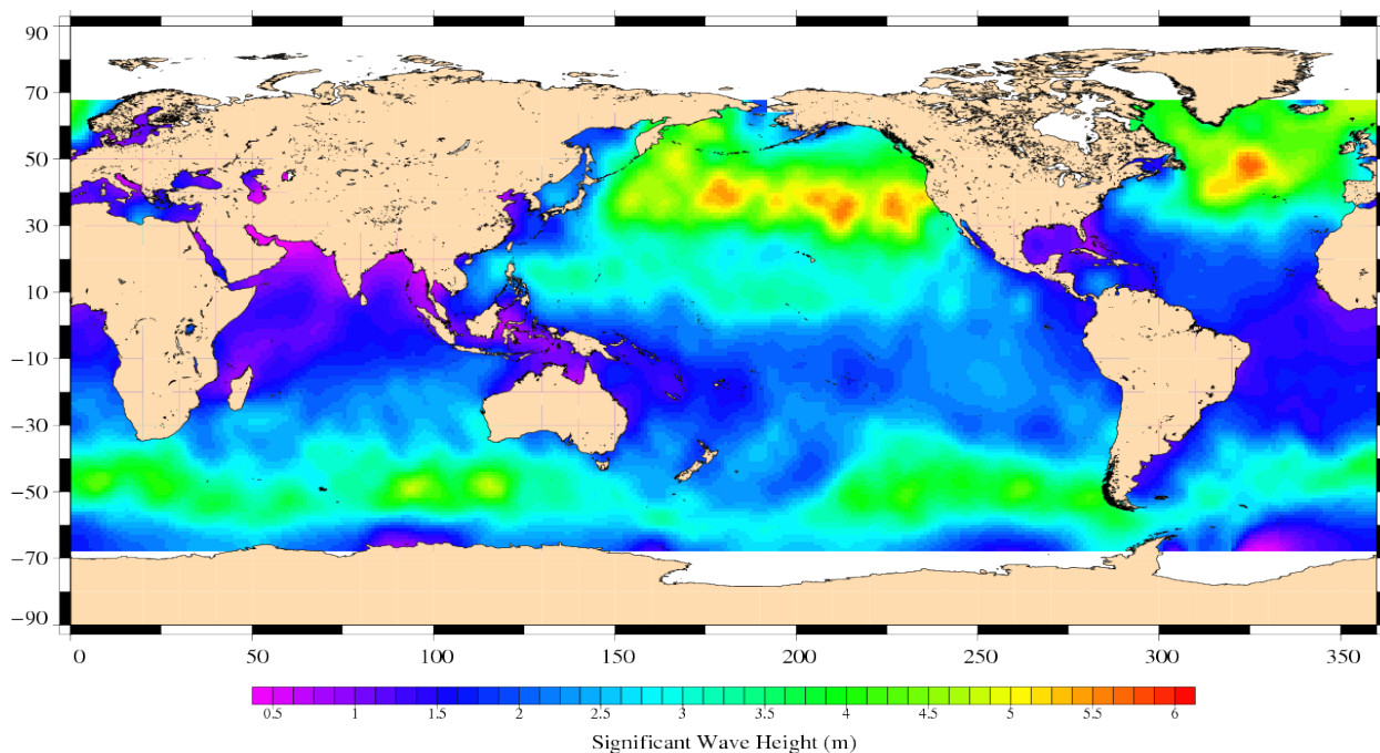
Jason-1 Cycle 296 13/01/2010 – 23/01/2010
