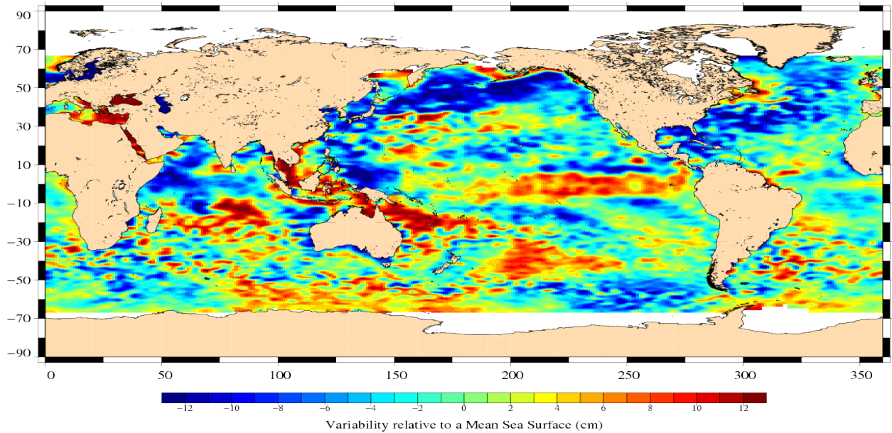
Jason-1 Cycle 296 13/01/2010 – 23/01/2010
