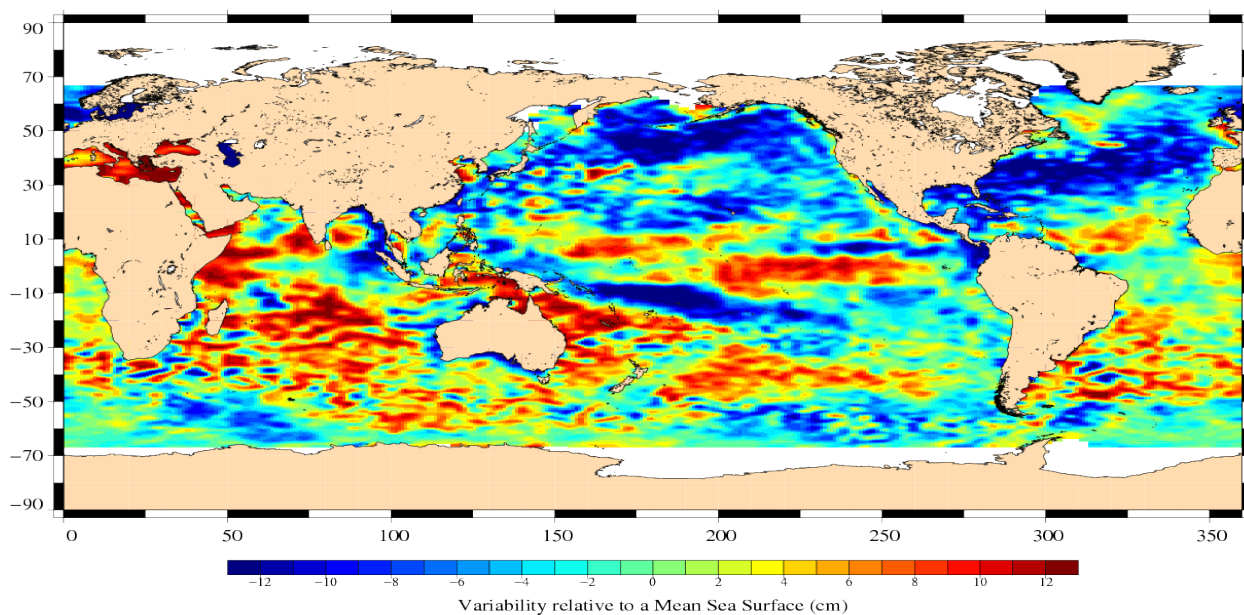
Jason-1 Cycle 300 22/02/2010 – 03/03/2010
