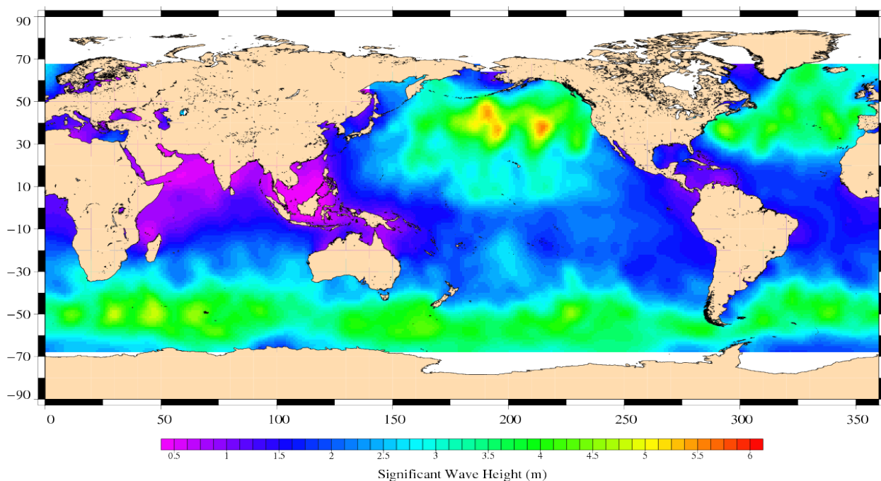
Jason-1 Cycle 300 22/02/2010 – 03/03/2010
