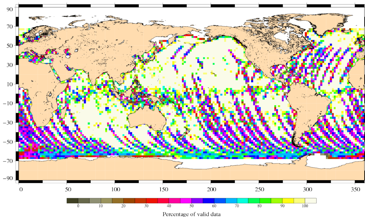
Percentage of valid data relative to the nominal pass Jason-1 Cycle 304 (02/04/2010 / 12/04/2010)
