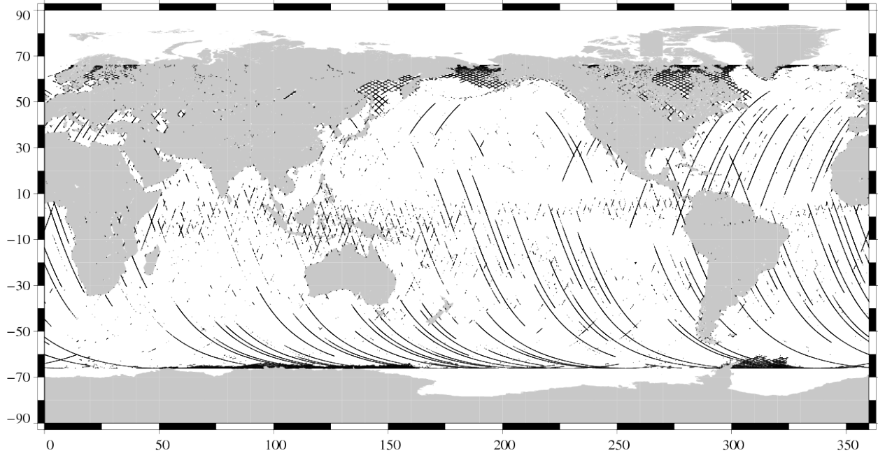
Valid data Jason-1 Cycle 304 (02/04/2010 / 12/04/2010)
