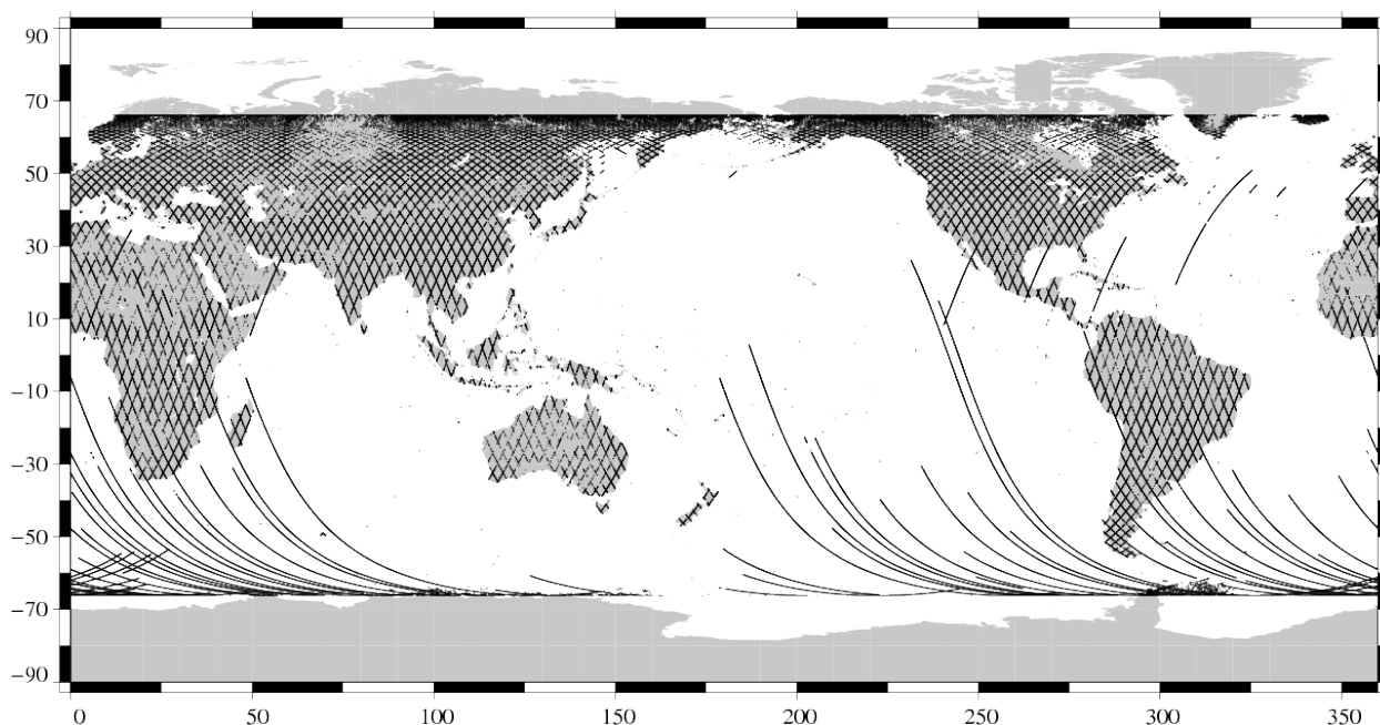
Missing measurements Jason-1 Cycle 304 (02/04/2010 / 12/04/2010)
