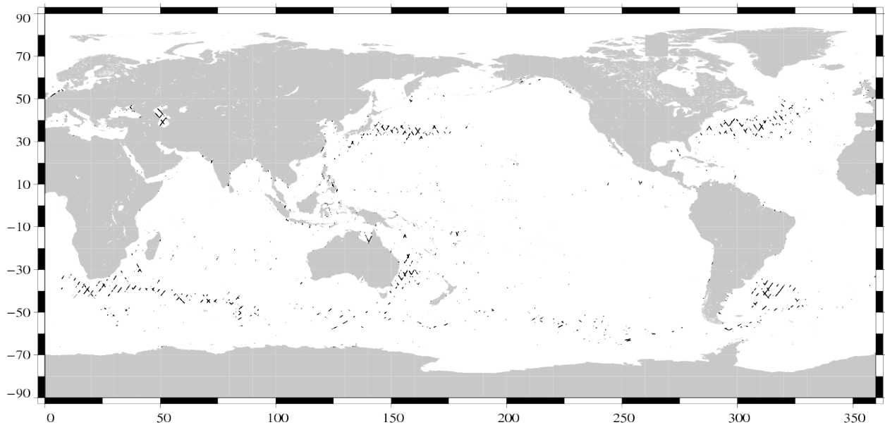
Valid data: (SSH – MSS) differences greater than 30 cm Jason-1 Cycle 304 (02/04/2010 / 12/04/2010)
