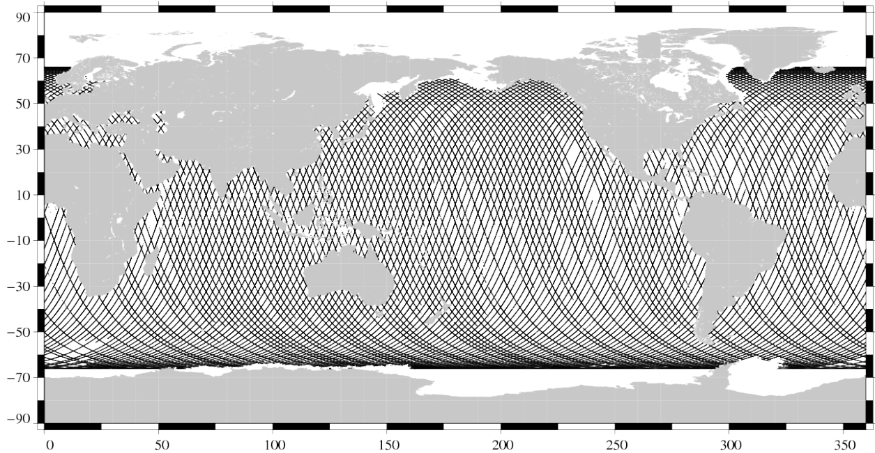
Valid data Jason-1 Cycle 304 (02/04/2010 / 12/04/2010)
