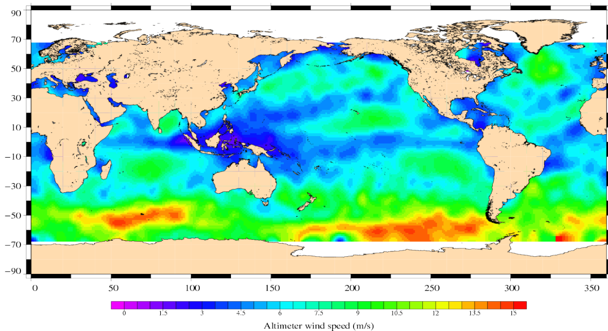
Jason-1 Cycle 309 22/05/2010 – 01/06/2010
