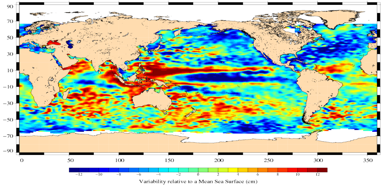
Jason-1 Cycle 309 22/05/2010 – 01/06/2010
