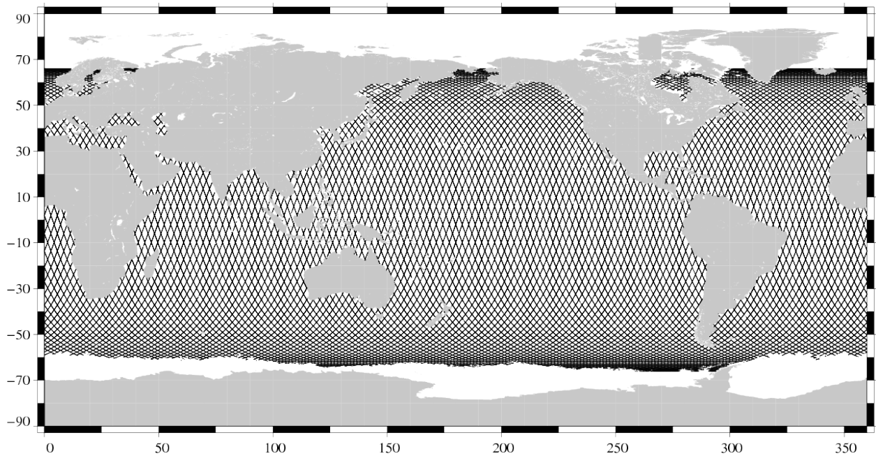
Valid data Jason-1 Cycle 313 (30/06/2010 / 10/07/2010)
