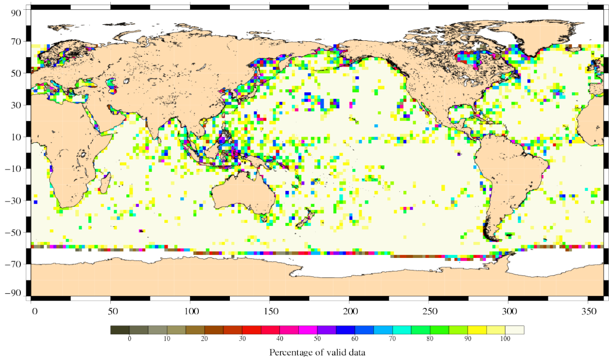
Percentage of valid data relative to the nominal pass Jason-1 Cycle 313 (30/06/2010 / 10/07/2010)
