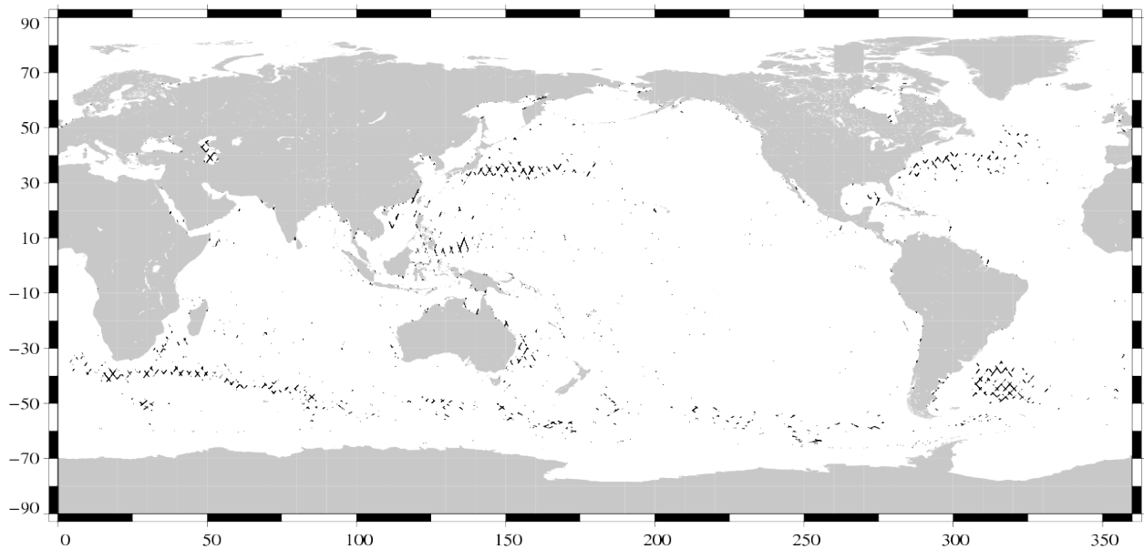
Valid data: (SSH – MSS) differences greater than 30 cm Jason-1 Cycle 313 (30/06/2010 / 10/07/2010)
