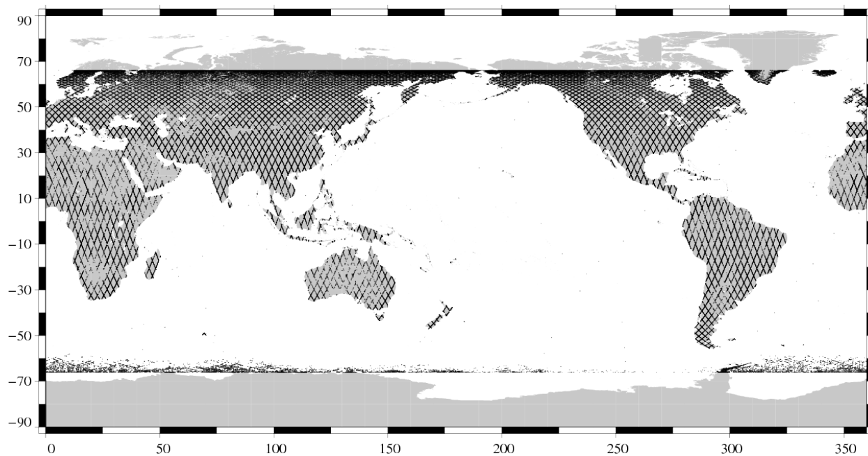
Missing measurements Jason-1 Cycle 313 (30/06/2010 / 10/07/2010)
