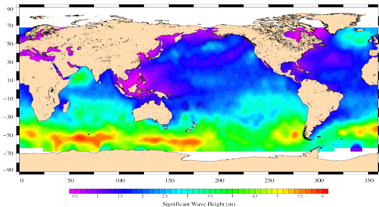
Jason-1 Cycle 313 30/06/2010 – 10/07/2010
