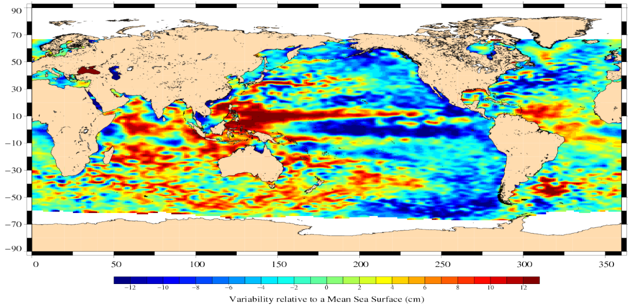
Jason-1 Cycle 313 30/06/2010 – 10/07/2010
